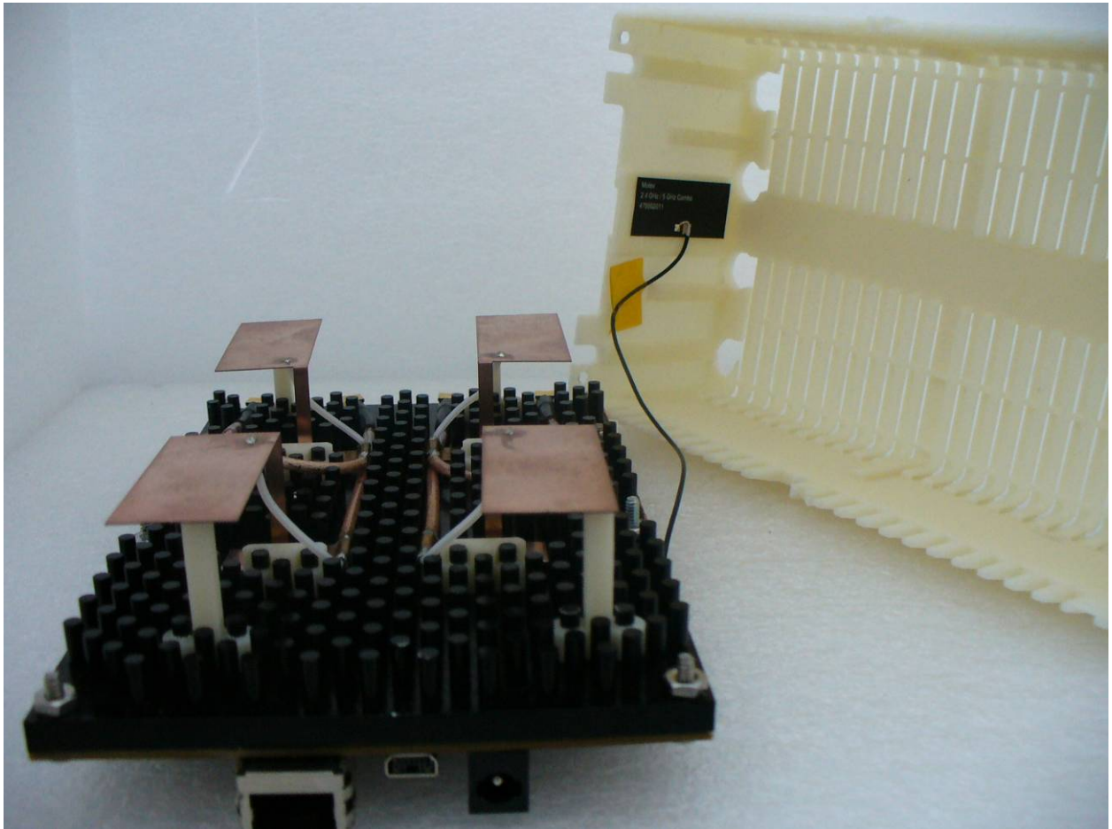
Figure 10: WLAN Antenna Location
