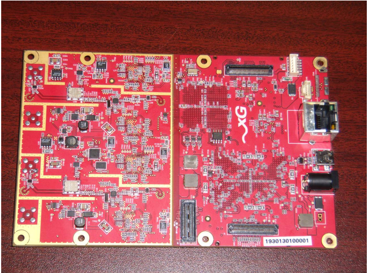
Figure 7: Main Board – Bottom View without Shielding
