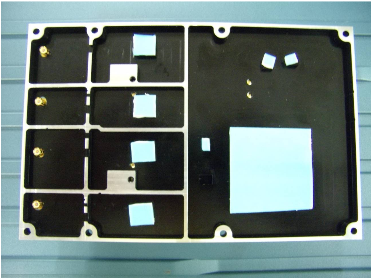
Figure 5: Top Shield Heat Sink Antenna – Bottom View
