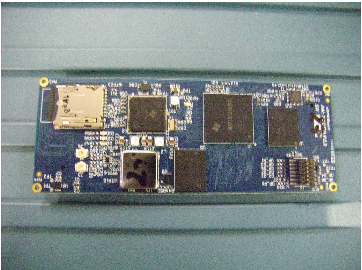
Figure 1: DPM Board – Top View with shielding
