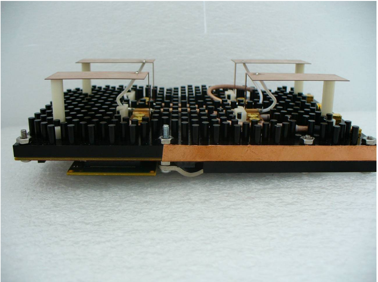
Figure 11: Assembled View with Modifications Implemented
