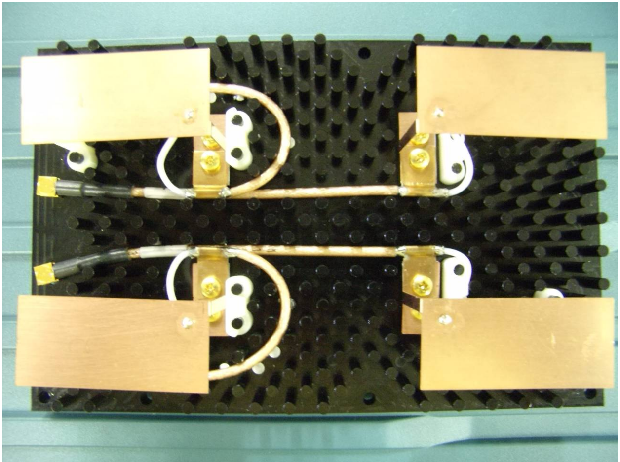
Figure 4: Top Shield Heat Sink Antenna – Top View
