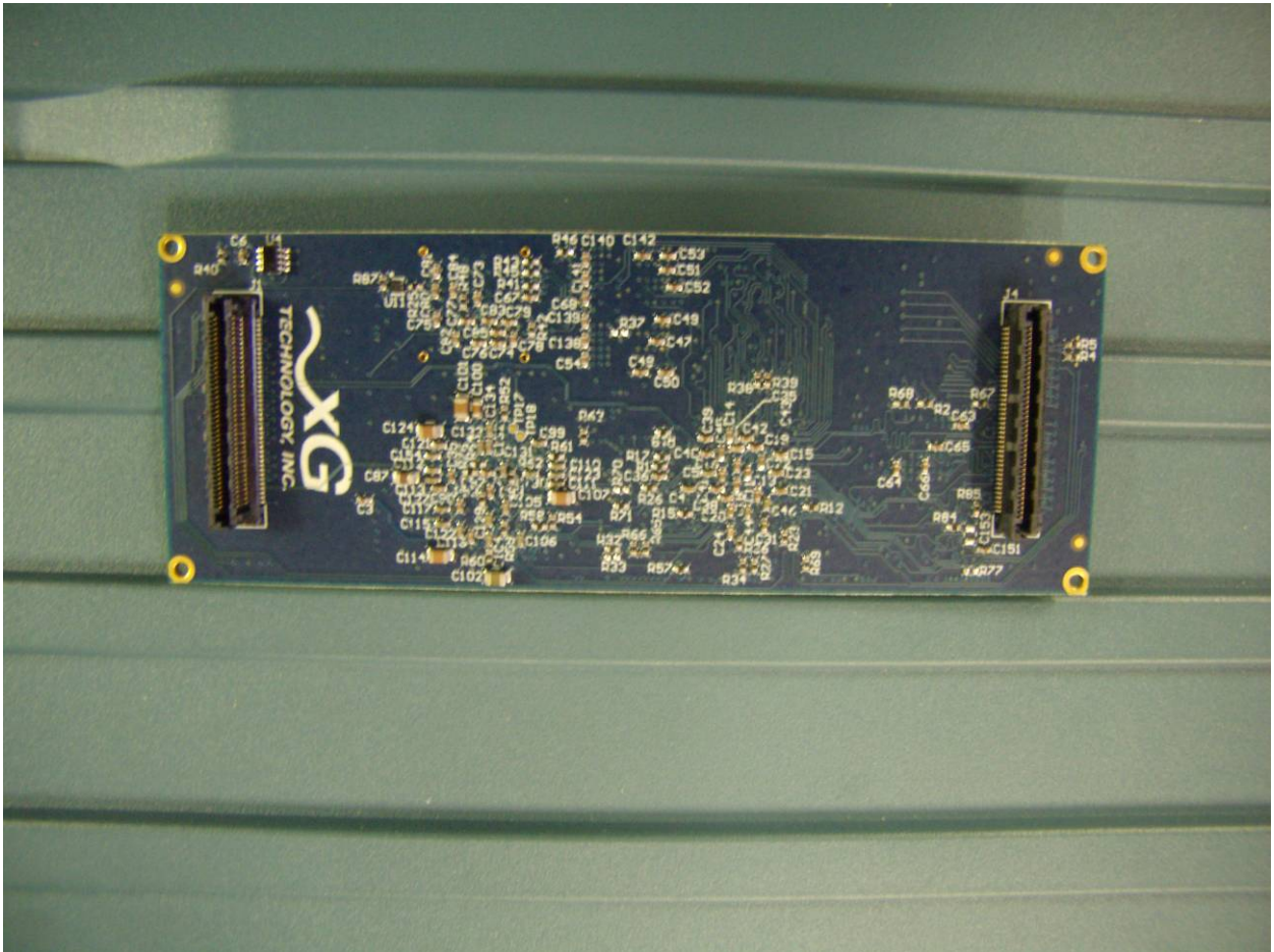
Figure 3: DPM Board – Bottom View
