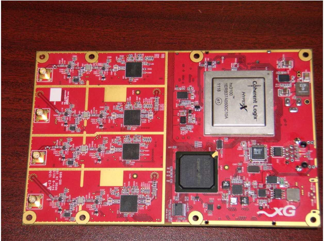
Figure 6: Main Board – Top View without Shielding
