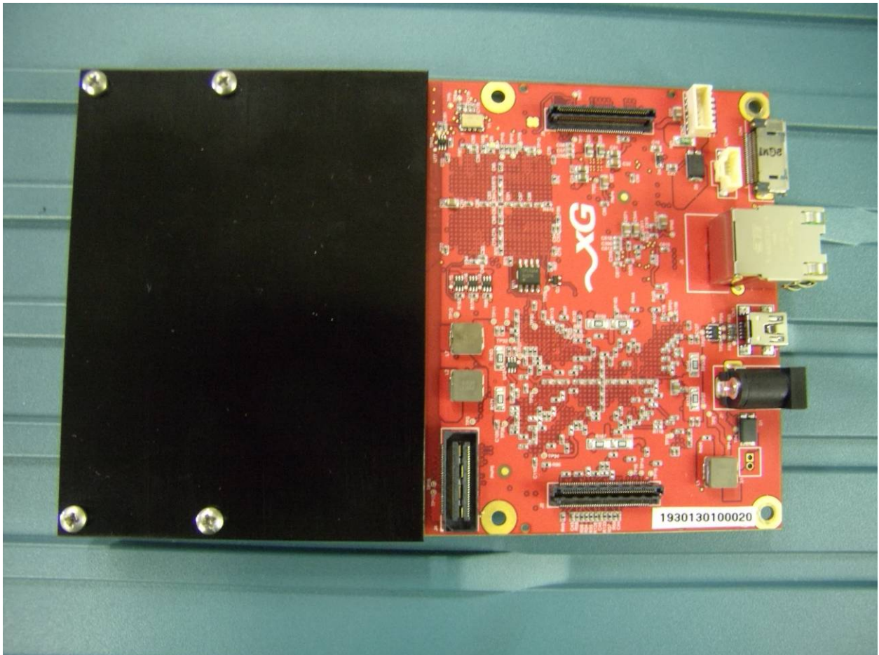
Figure 8: Main Board – Bottom View with Shielding
