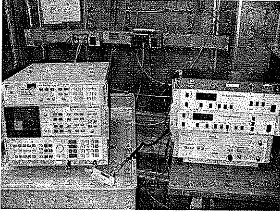
Photographs 5 and 6: Bandwidth and Power Measurement Setup
