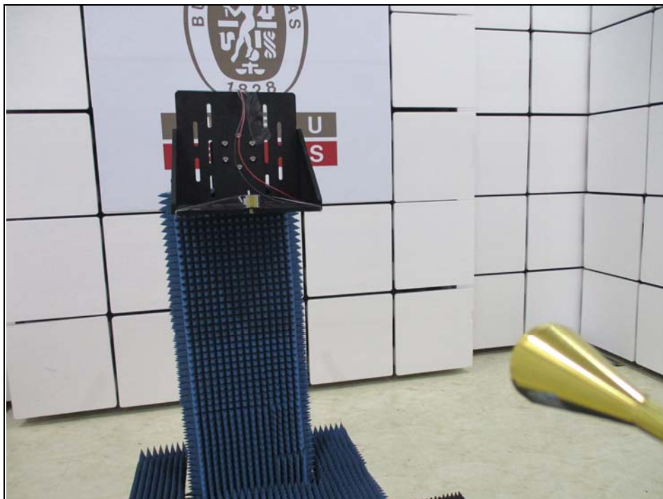
Radiated Emission Test (50~75GHz)
