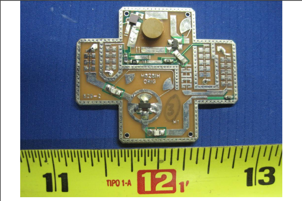
EUT PCBA – Component View
