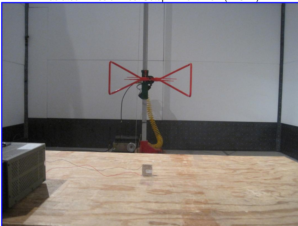
Radiated Emission Test Setup – Rear View (<1GHz)
