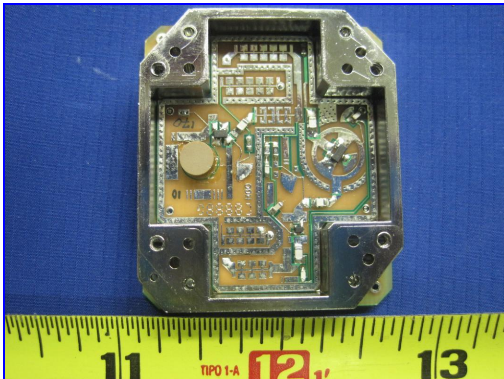
EUT PCBA – Cover Off View
