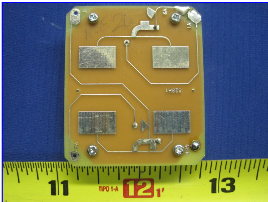
Antenna View
