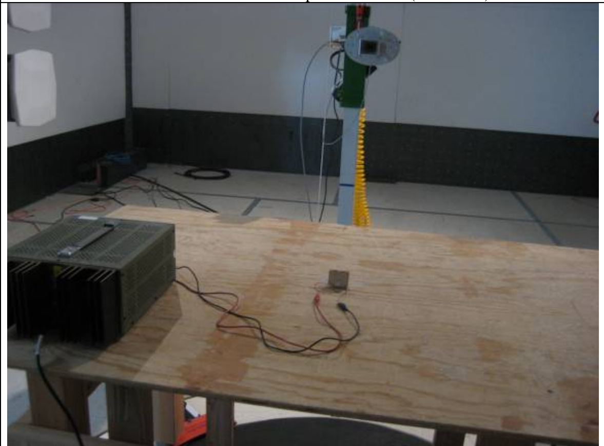
Radiated Emission Test Setup – Rear View (18-40GHz)
