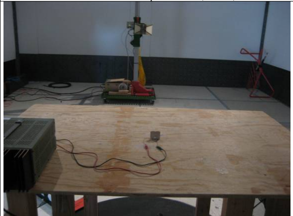
Radiated Emission Test Setup – Rear View (1-18GHz)
