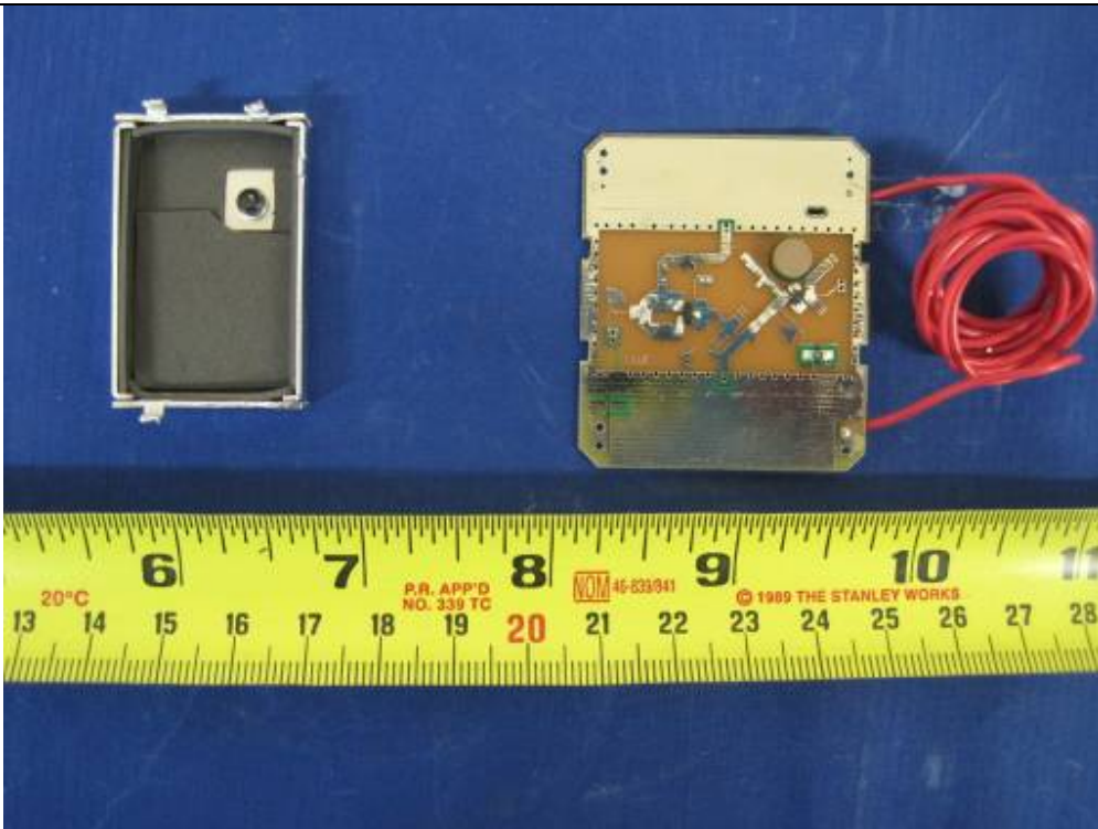
EUT PCB– without RF shield View
