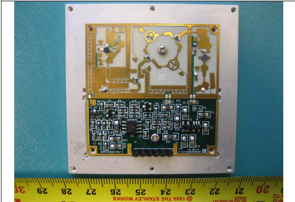
EUT PCBA – Component View with Plate
