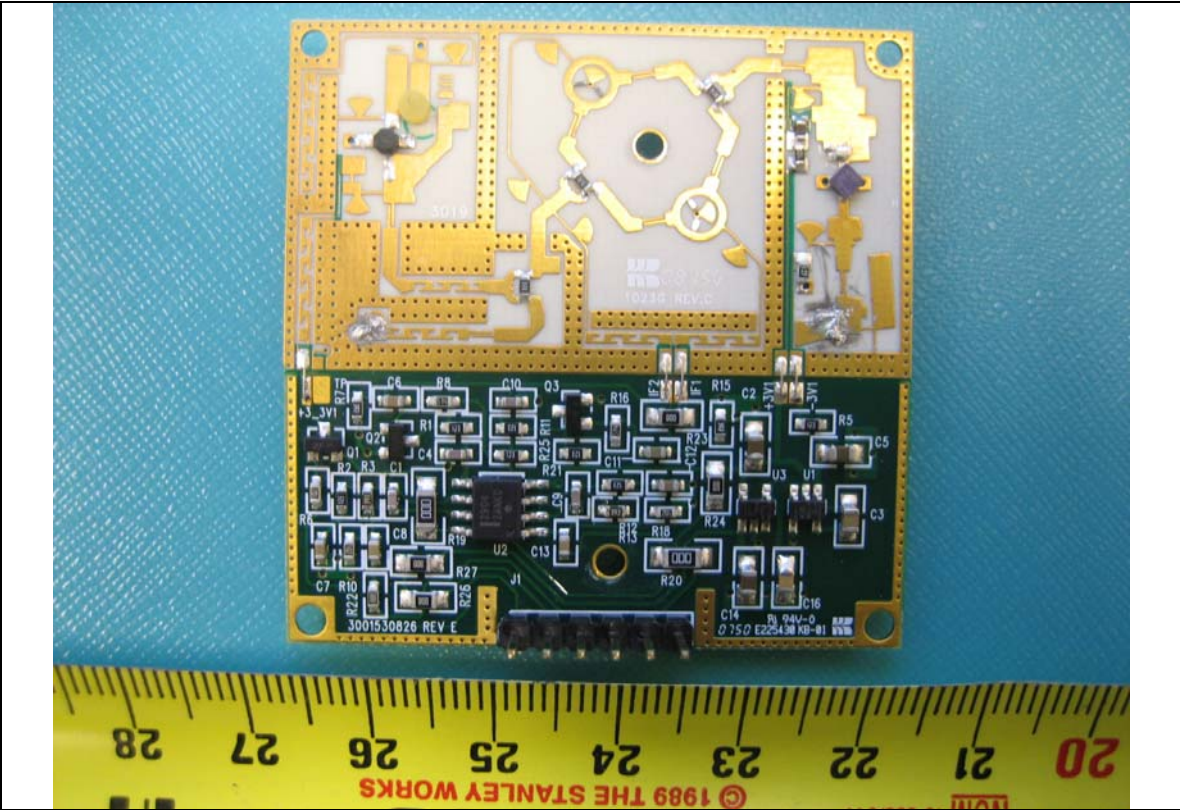
EUT PCBA – Component View
