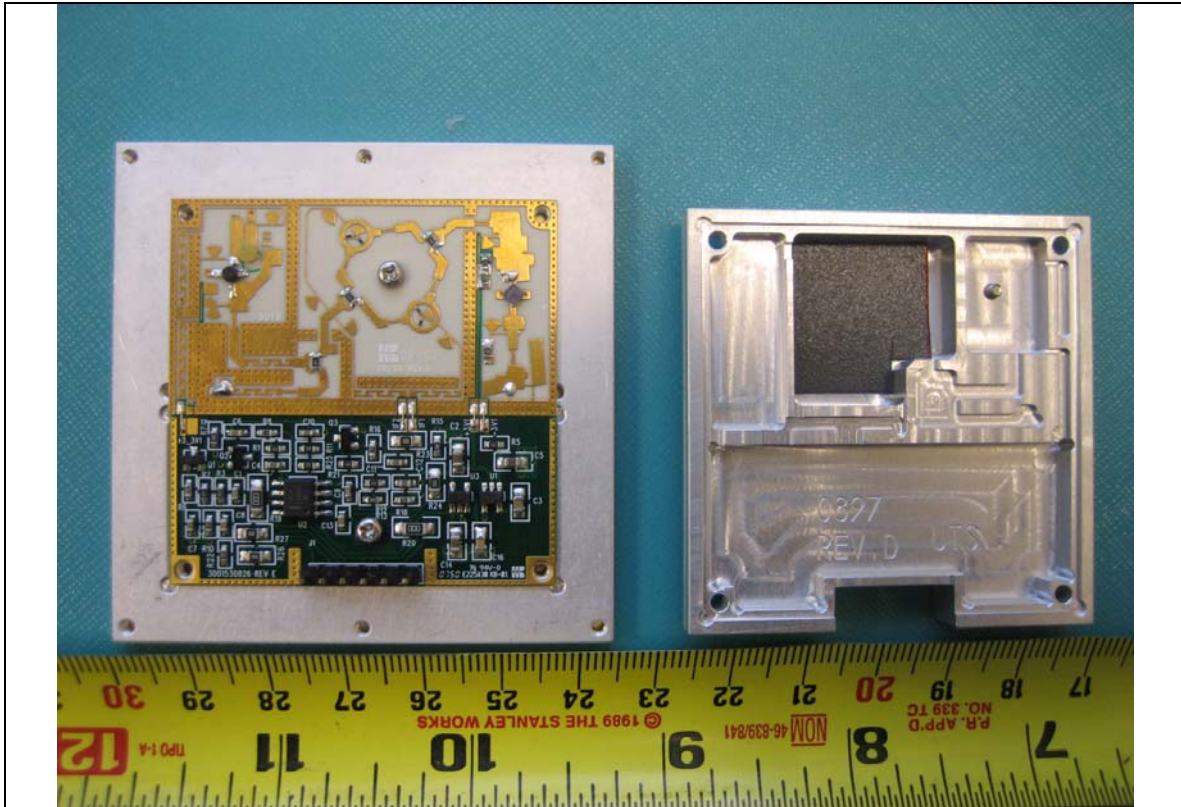
EUT PCBA – Cover Off View
