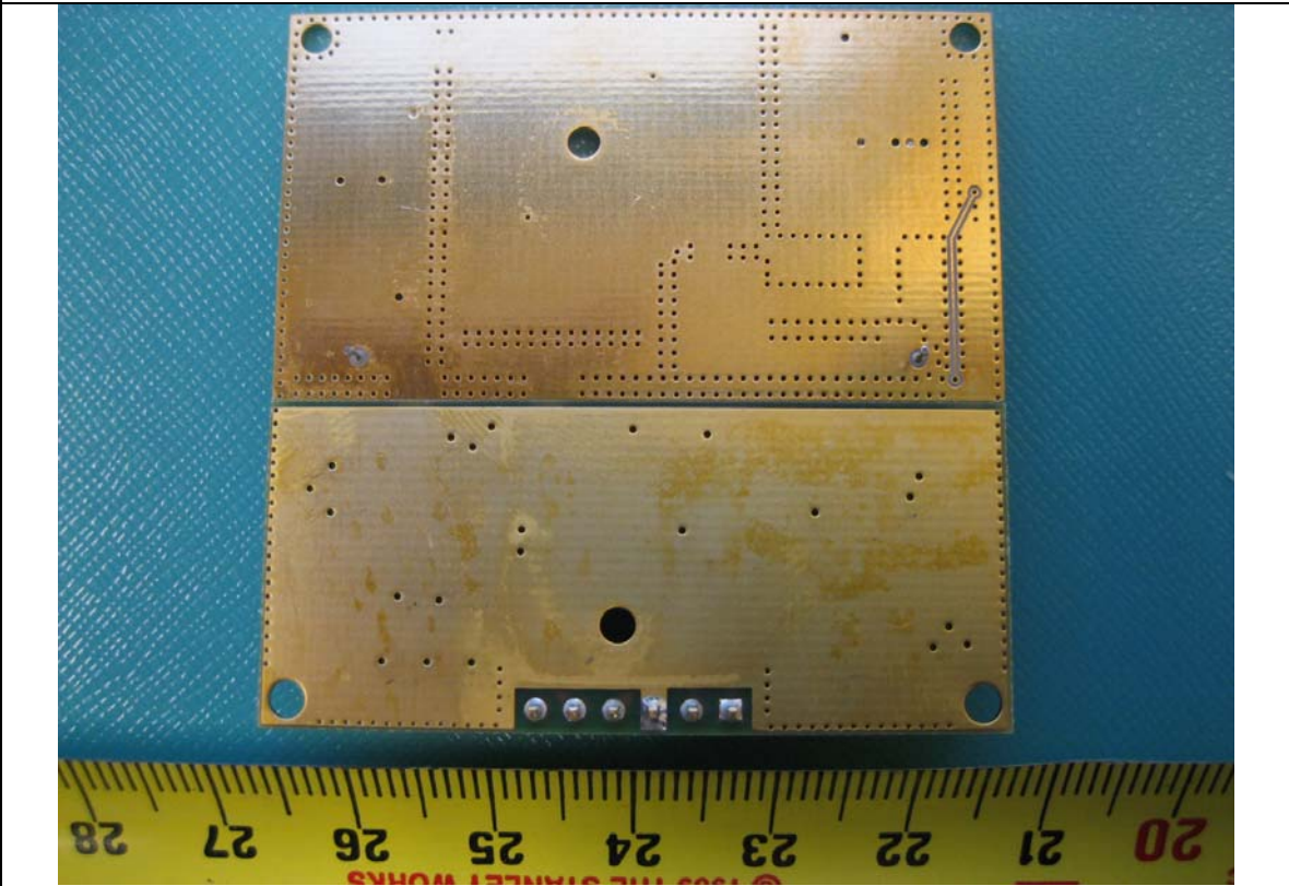
EUT PCBA – Solder View
