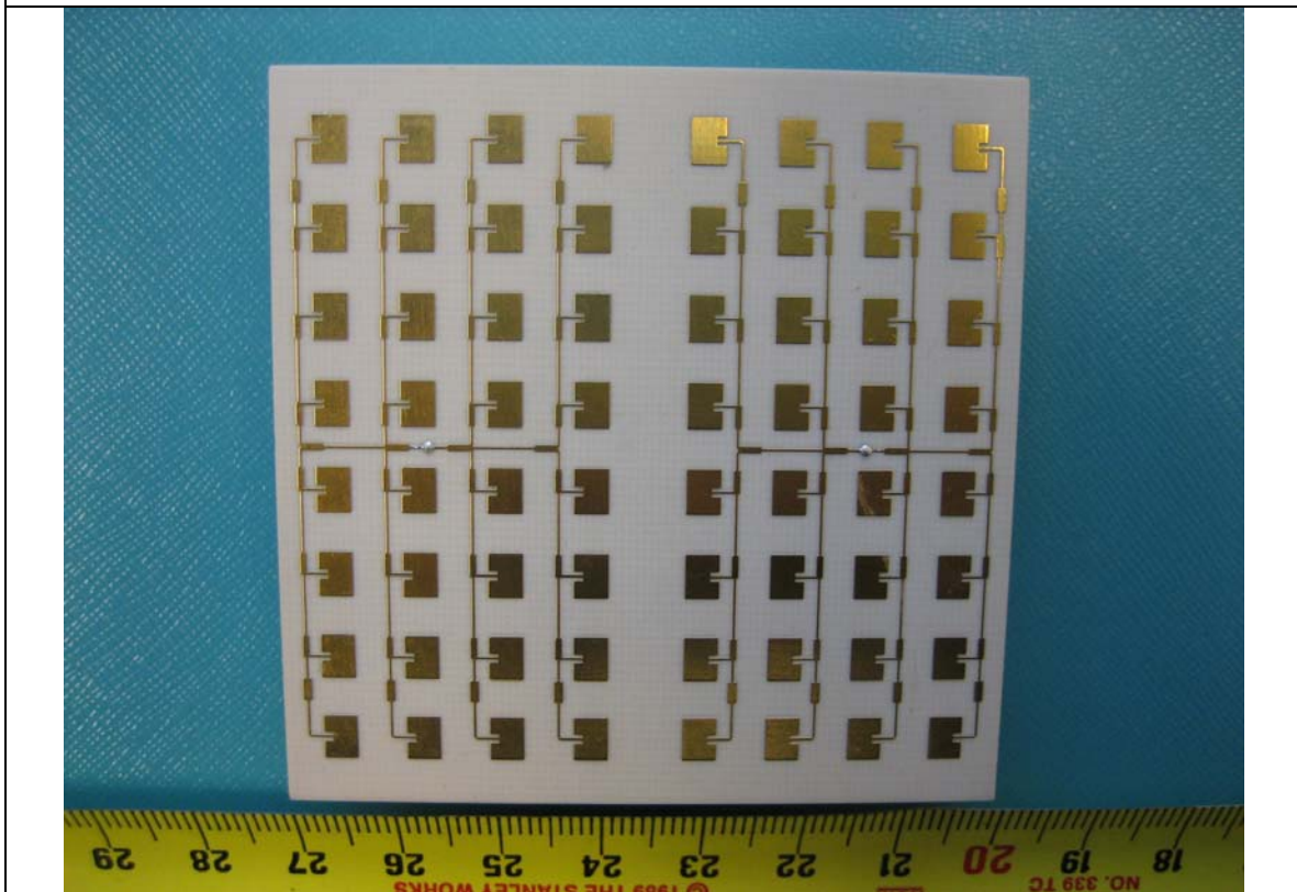
Antenna View
