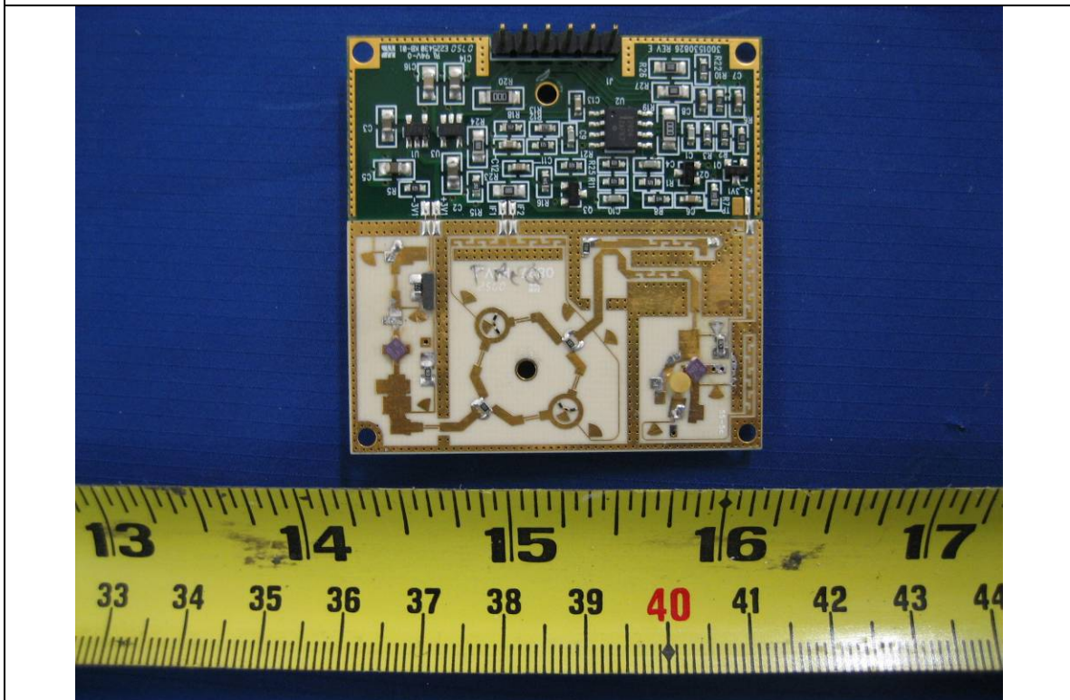
EUT PCBA – Component View
