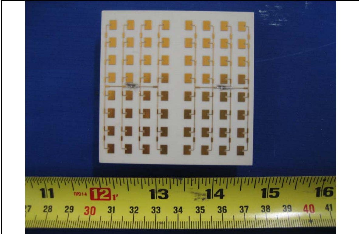
Antenna View
