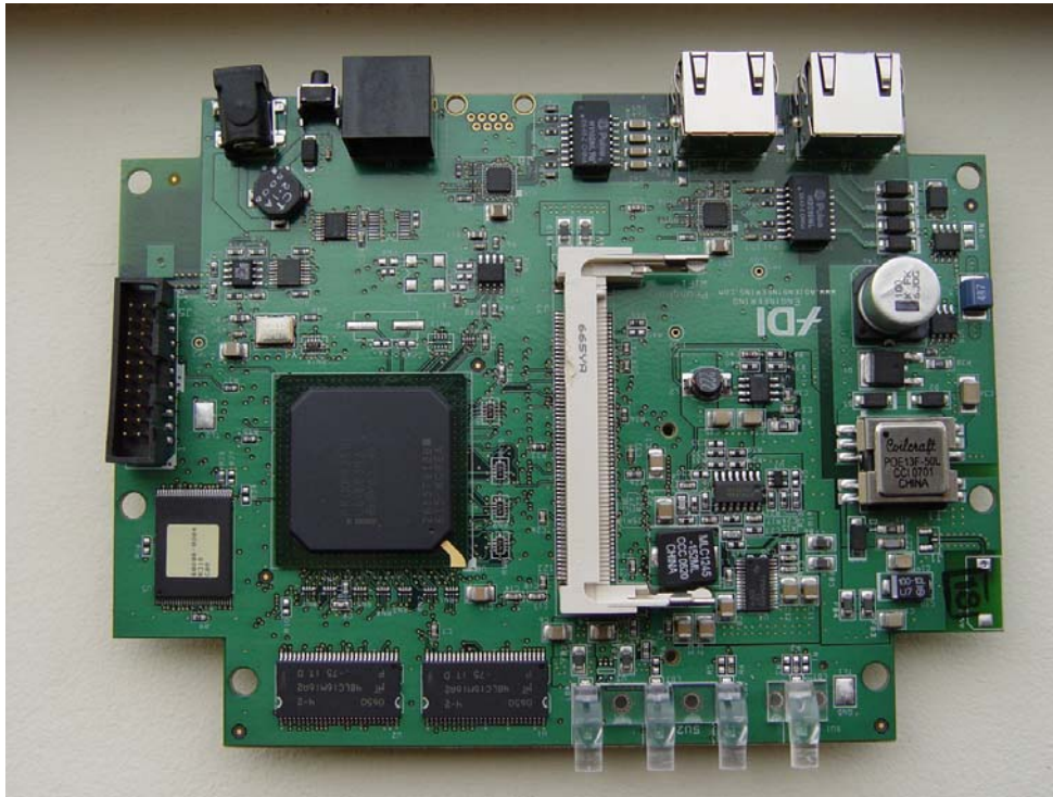
Motherboard Bottom
