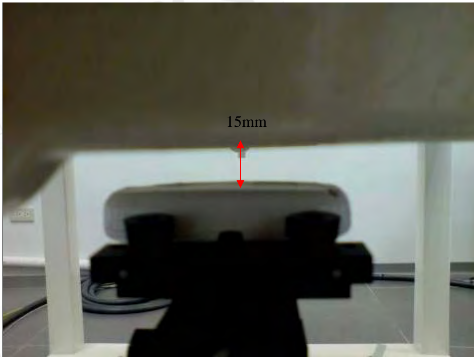
Fig.5 Back of EUT is paralleled with flat phantom, and spacing between EUT and Phantom is 15mm.
