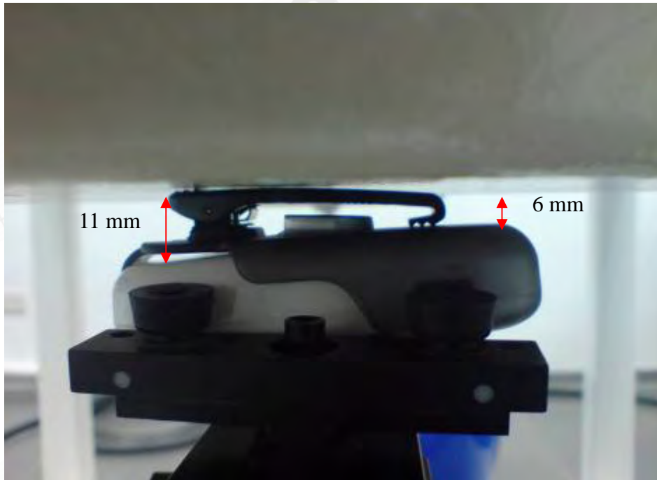
Fig.3 Back of EUT is paralleled with flat phantom, and contact it
