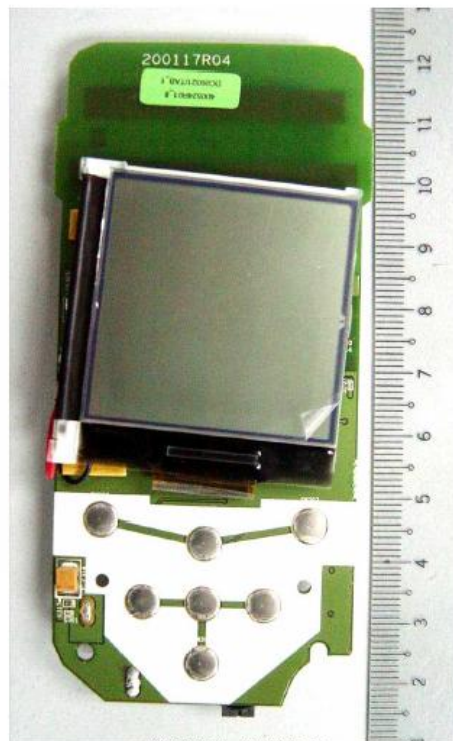
EUT PCB View 1 (with LCD)
