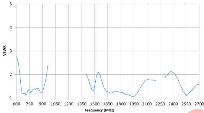
VSWR (600-2700 MHz)
