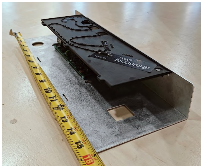
Figure 1– DUT Top and right view
