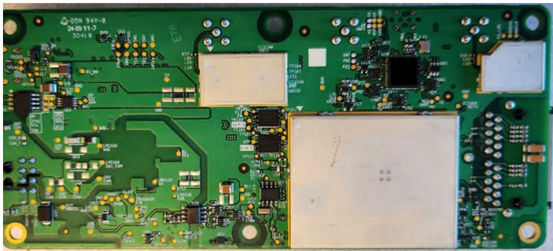
Figure 3: PCB Bottom
