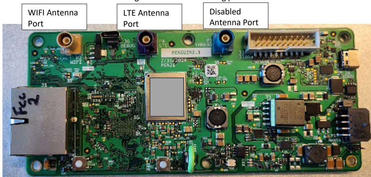
Figure 2: PCB Top
