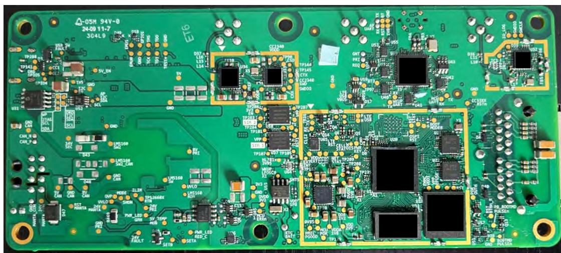
Figure 4: PCB Bottom with shields removed
