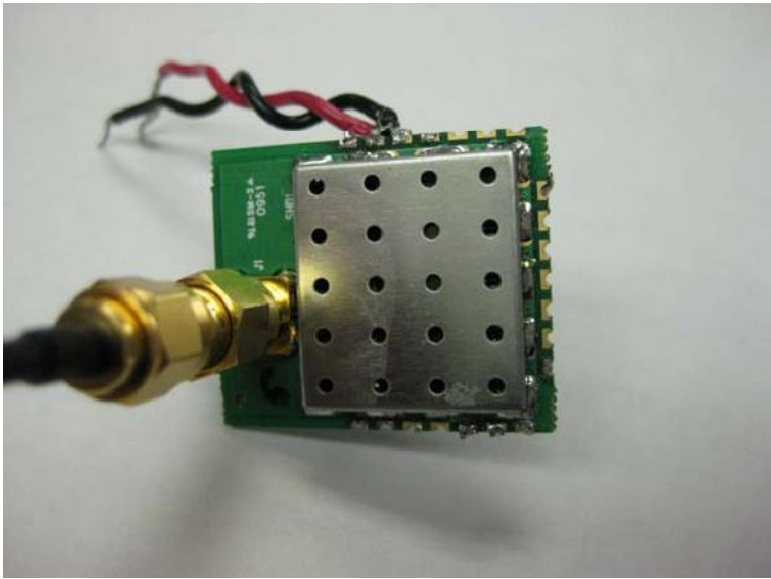
Dipole antenna board side connections
