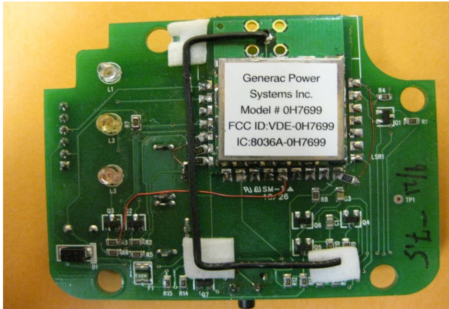
Board with custom wire antenna
