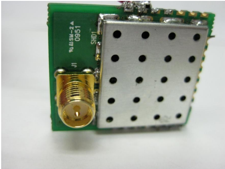
Dipole antenna board side connections (picture 3)
