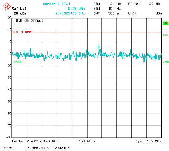
Low Channel (b-Mode) 2412 MHz
