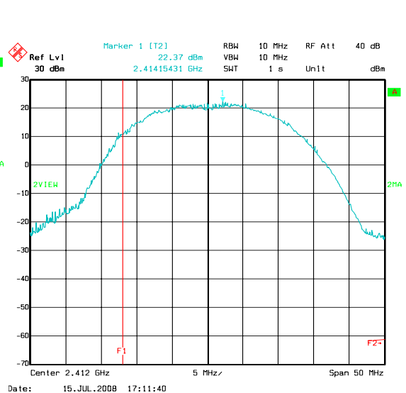
Low Channel (g-Mode) 2412 MHz
