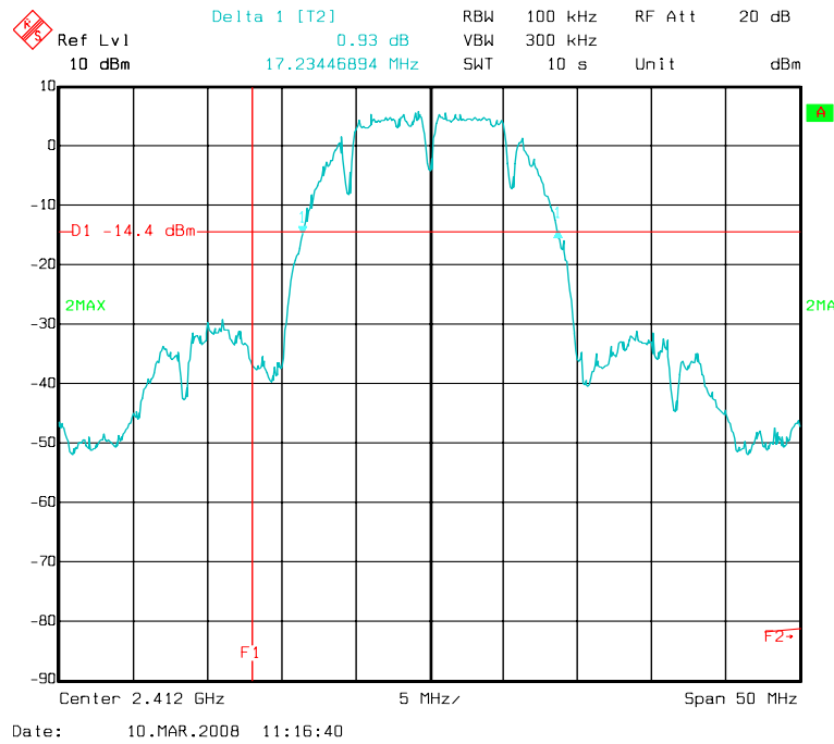
Low Channel (g-Mode) 2412 MHz (Peak Measurement)
