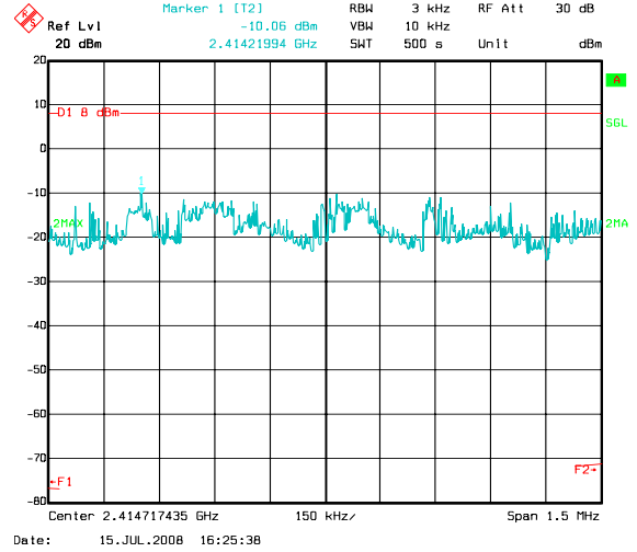
Low Channel (g-Mode) 2412 MHz
