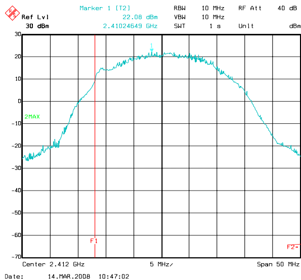
Low Channel (b-Mode) 2412 MHz
