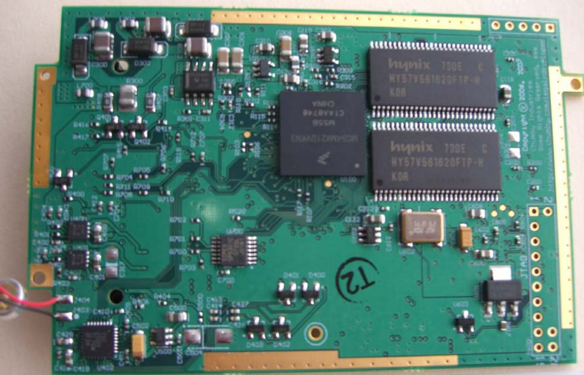
Motherboard CCA Topside
