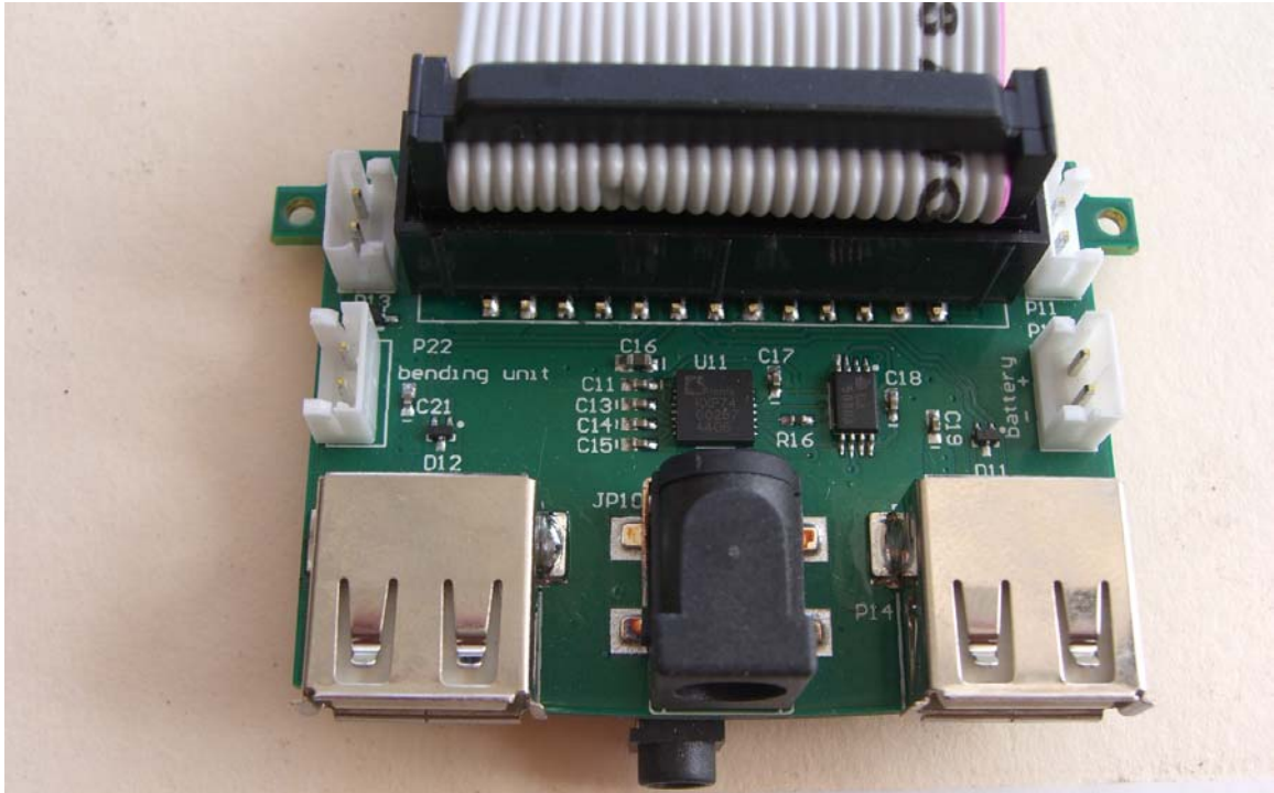
Daughterboard CCA Bottomside
