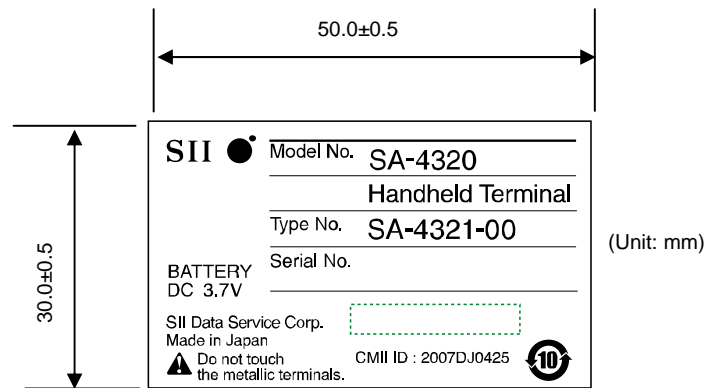
Fig. 10-2: Manufacturing control label
