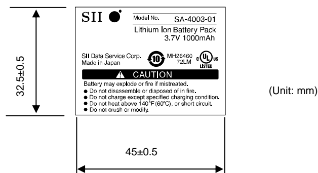
Fig.10-4: Battery pack label
