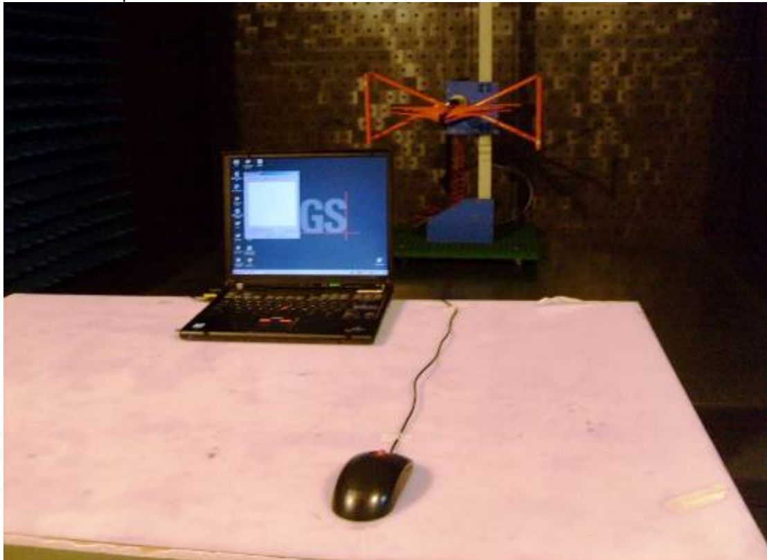
Radiated Spurious Emission
