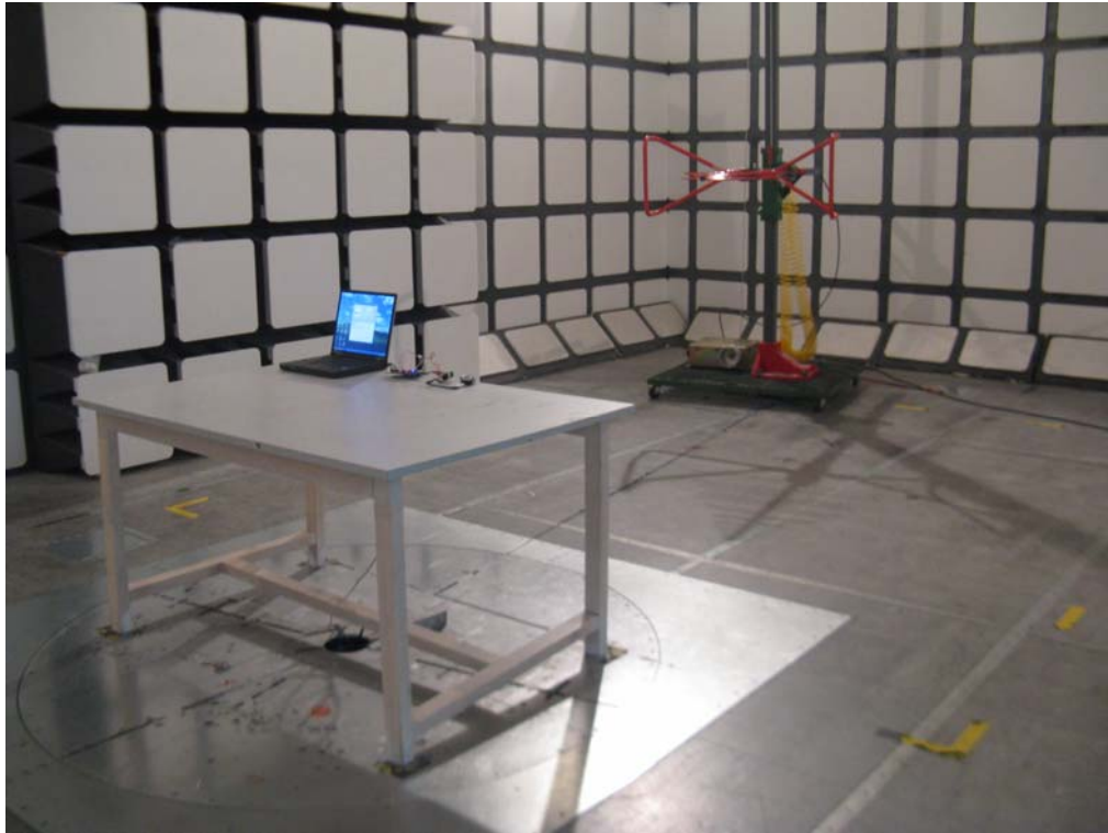
Transmitting mode: Radiated Emissions - Front View (30 -1000 MHz)
