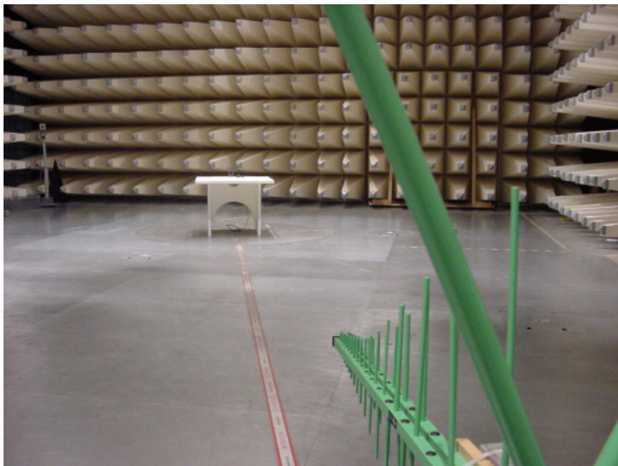
Photo 4 (Radiated Emissions):
