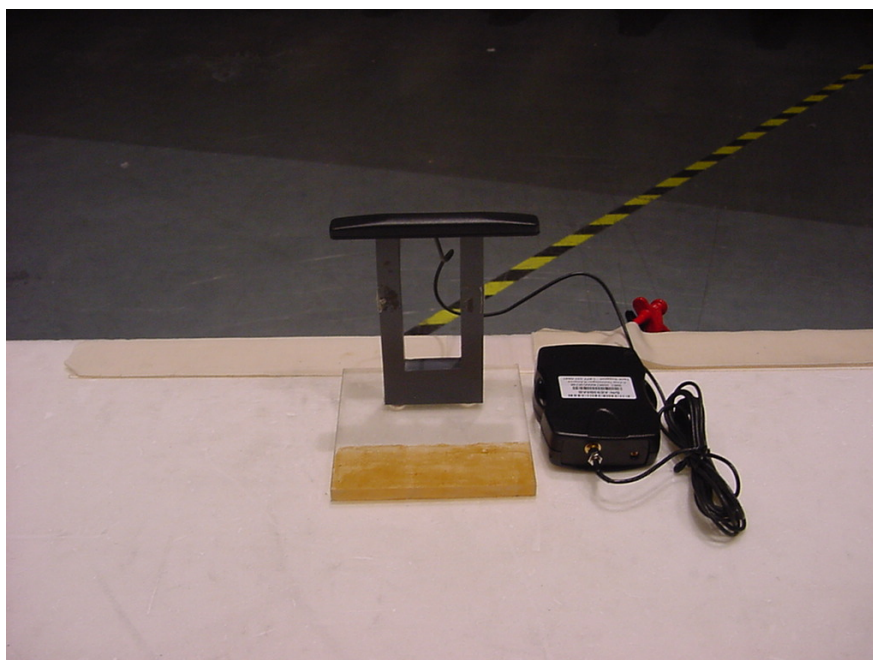
Photo 2 (Radiated Emissions):
