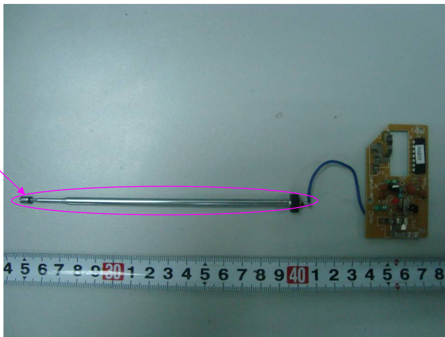
EUT – Mainboard and Antenna Top View
