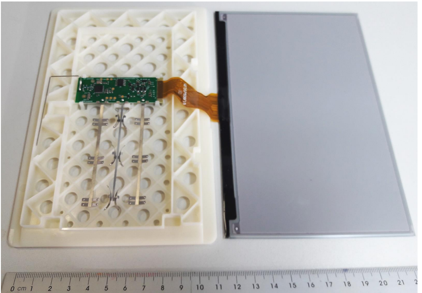
DISPLAY FOLDED OPEN, WITH FRONT & REAR COVERS REMOVED
