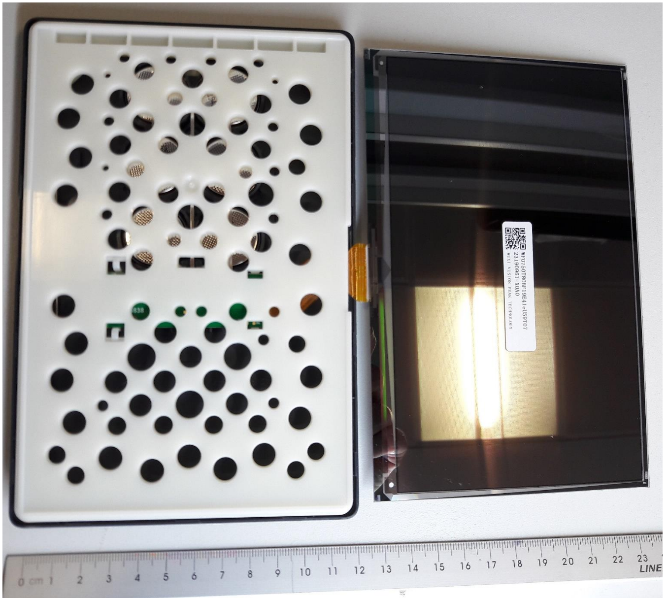
DISPLAY FOLDED OPEN SHOWING SPACER
