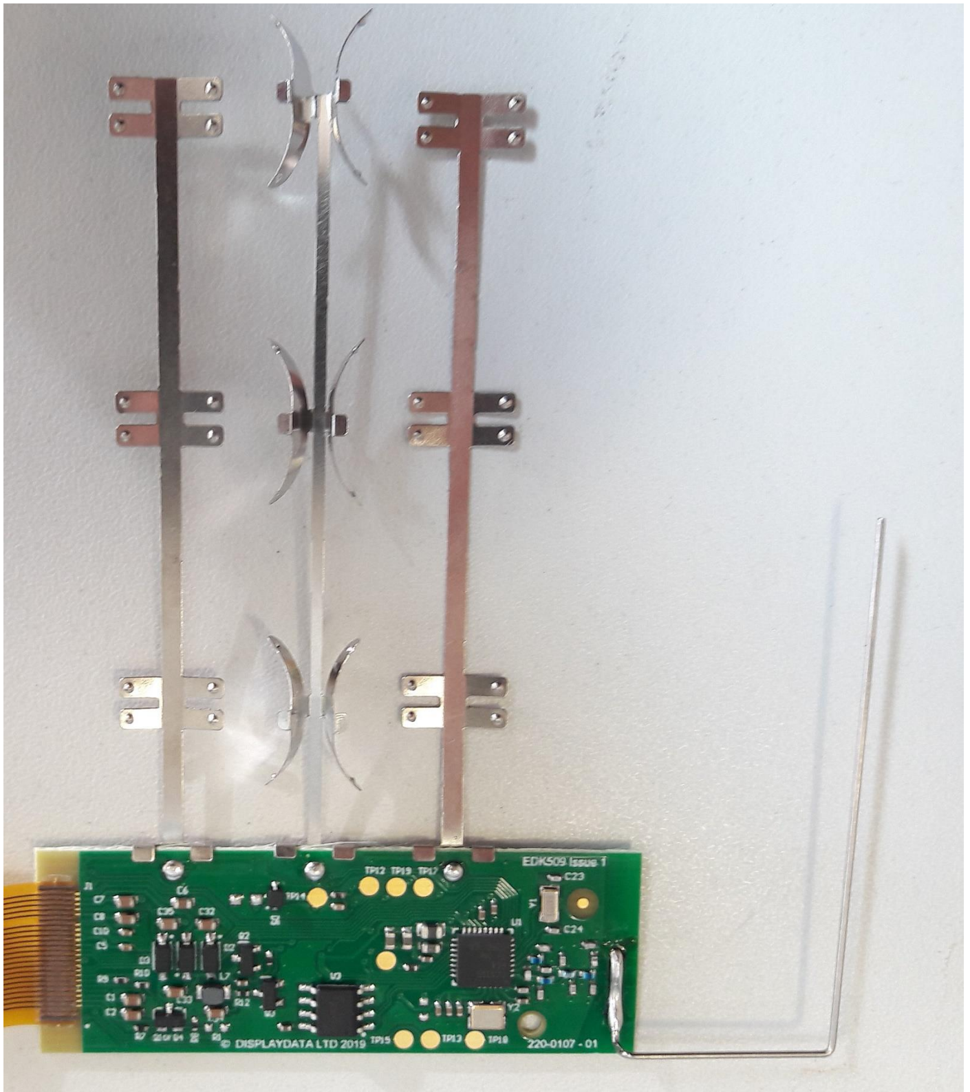
PCB COMPONENT SIDE
