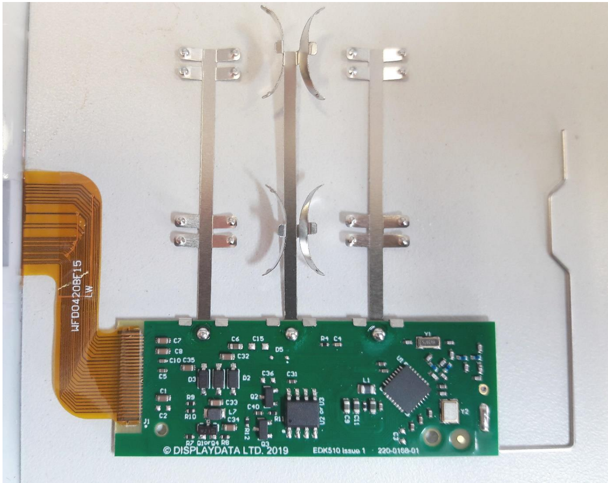
CLOSE-UP OF PCB COMPONENT SIDE
