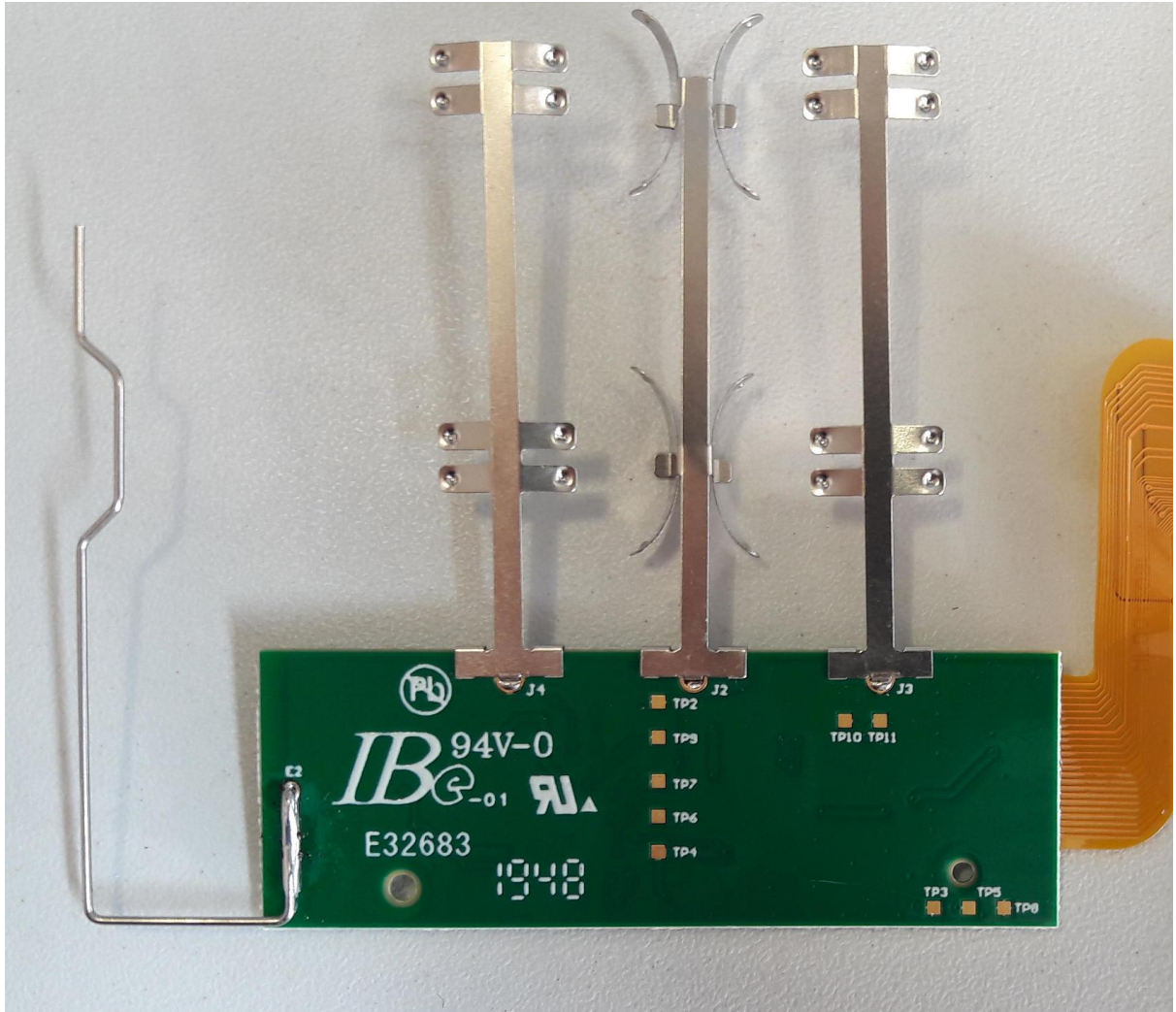
CLOSE UP OF PCB REAR SIDE
