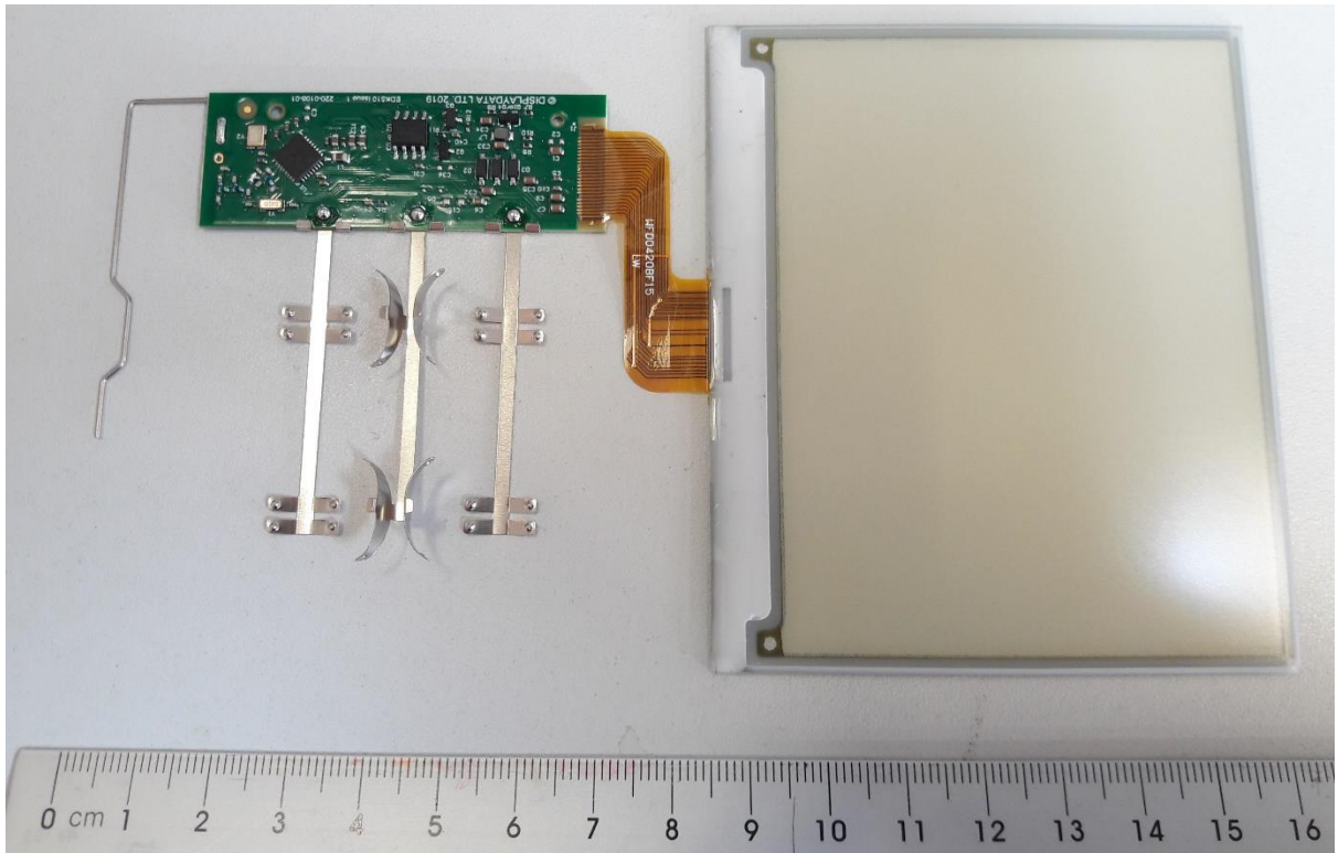
PCB AND DISPLAY
