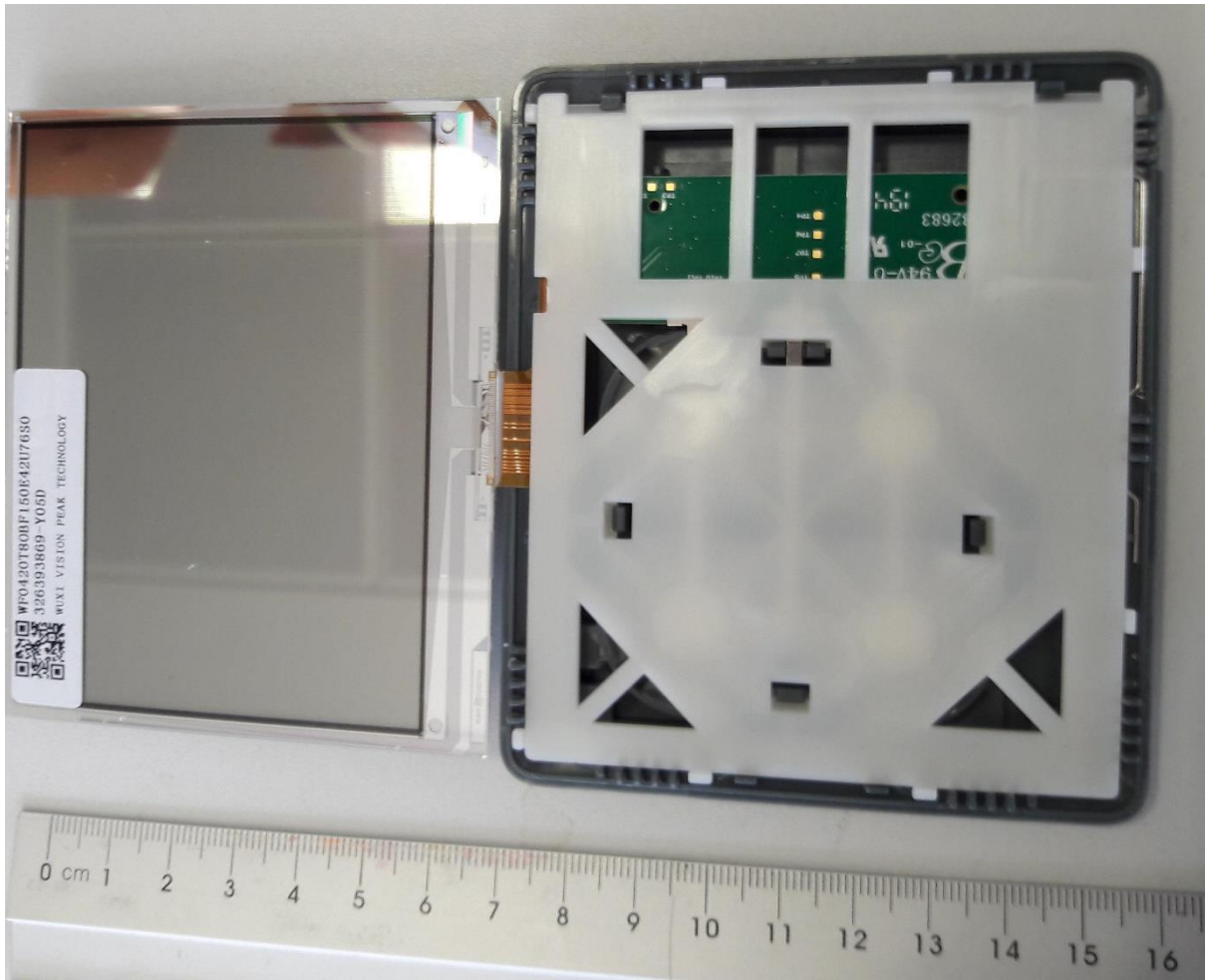
DISPLAY FOLDED OPEN SHOWING SPACER
