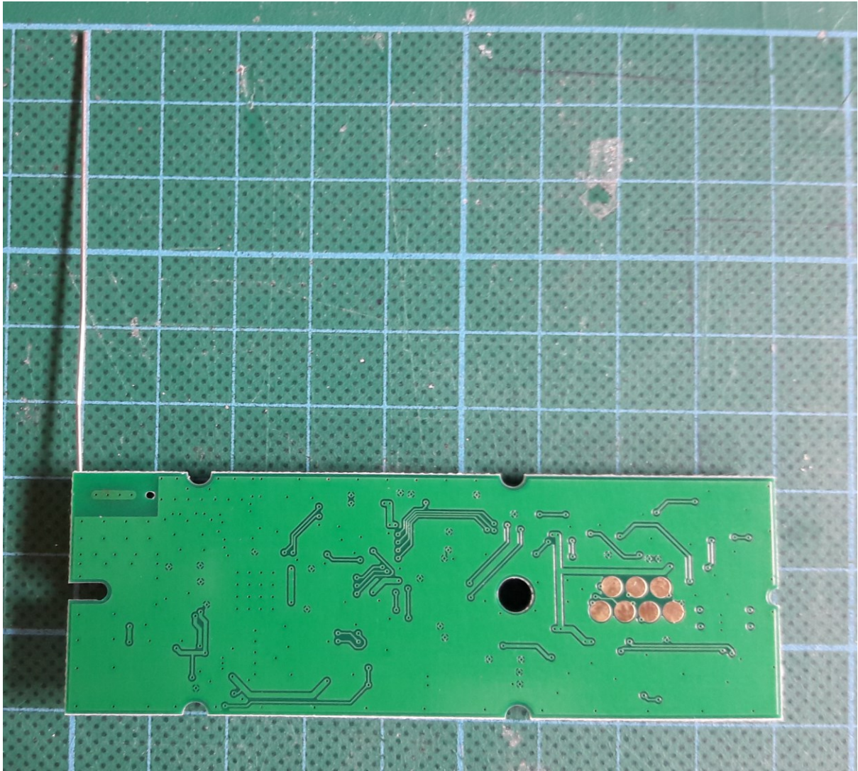
PCBA bottom side
