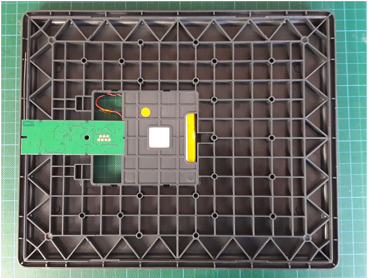
Front side: display glass removed (flex tails disconnected from PCBA)
