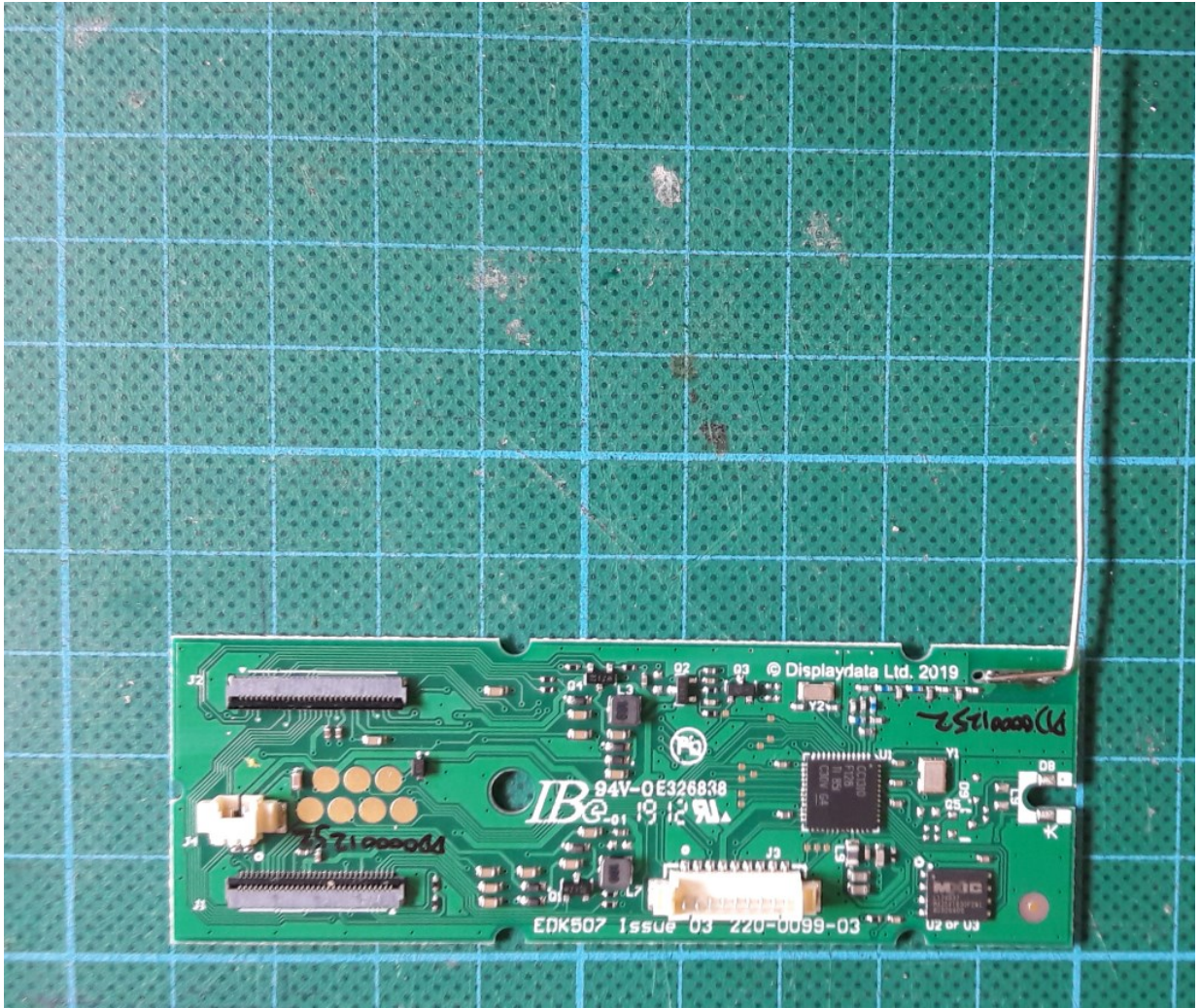
PCBA top/component side
