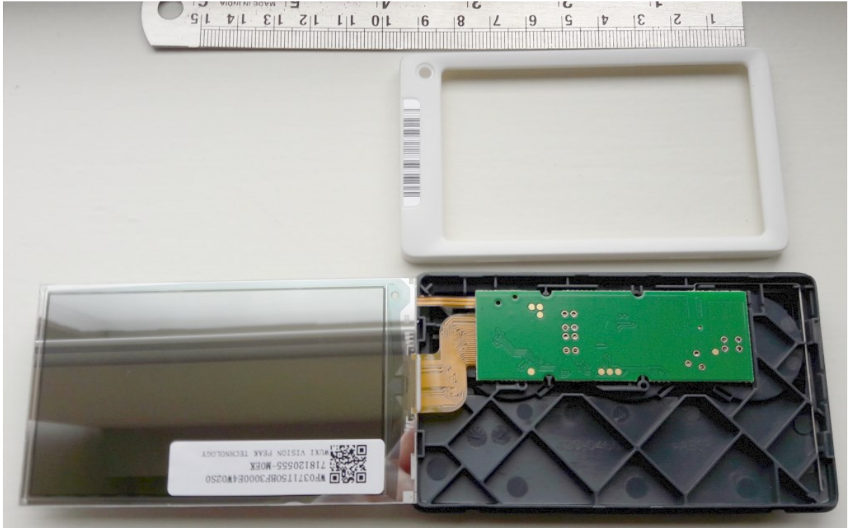
Front cover removed and display glass folded open
