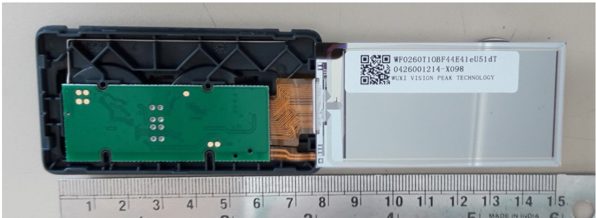
Front cover removed and display glass folded open
