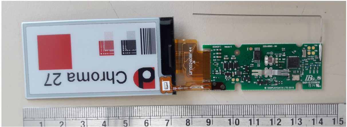
PCB and display glass front side
