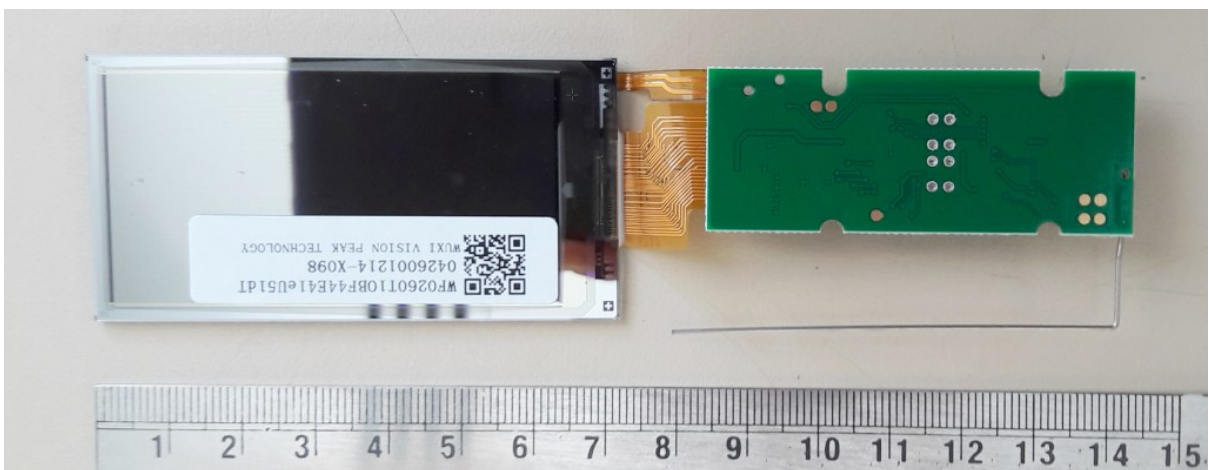
PCB and display glass rear side
