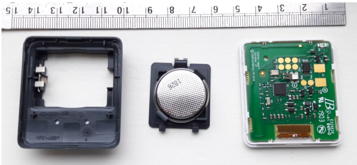
Showing PCB + Display folded into front cover
