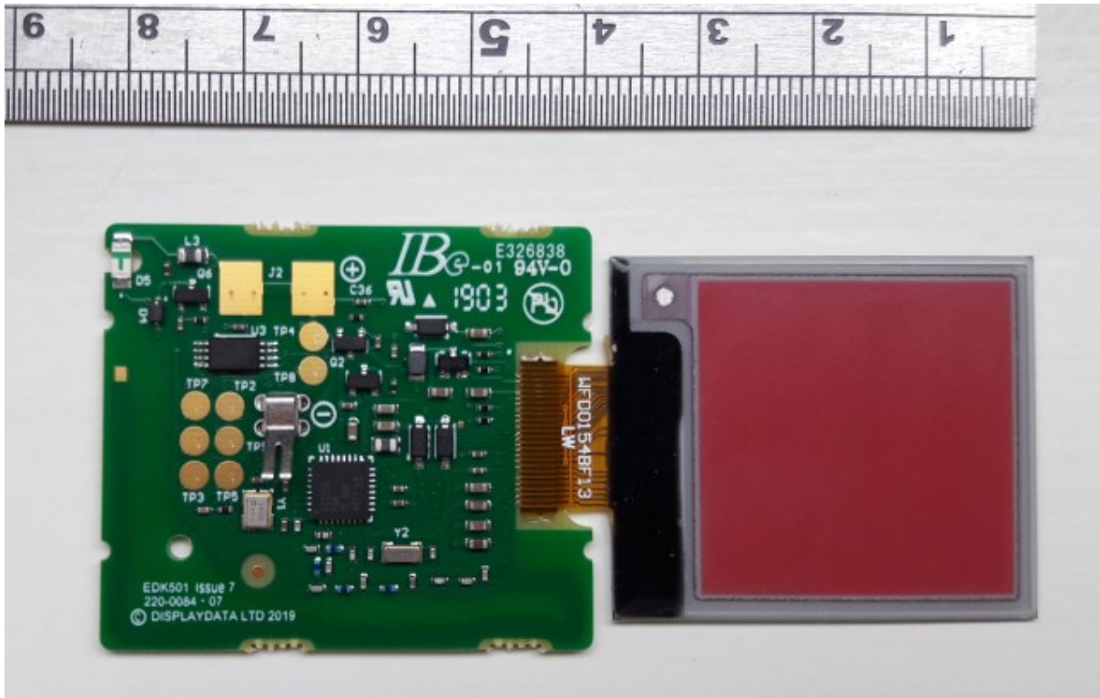
Display & PCB front view
