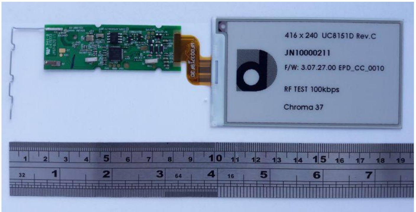
PCB component side with bonded display module:
