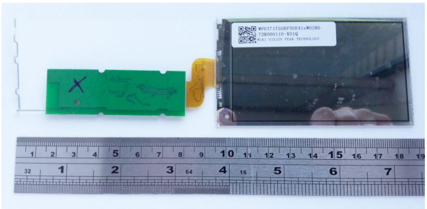
PCB component side with bonded display module:
