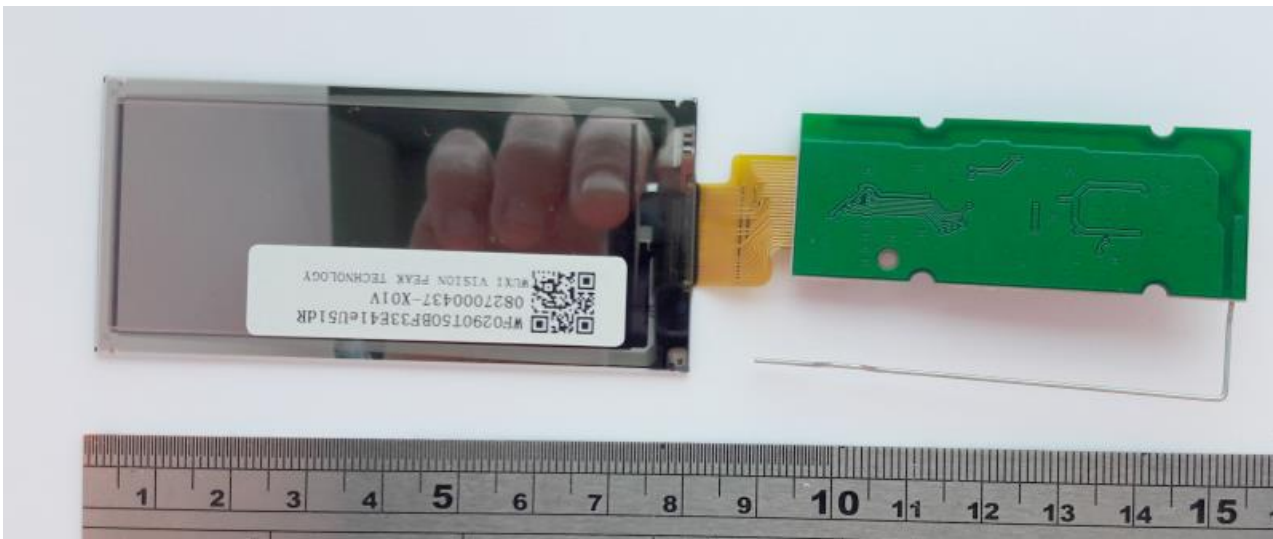
PCB rear side with bonded display and wire antenna:
