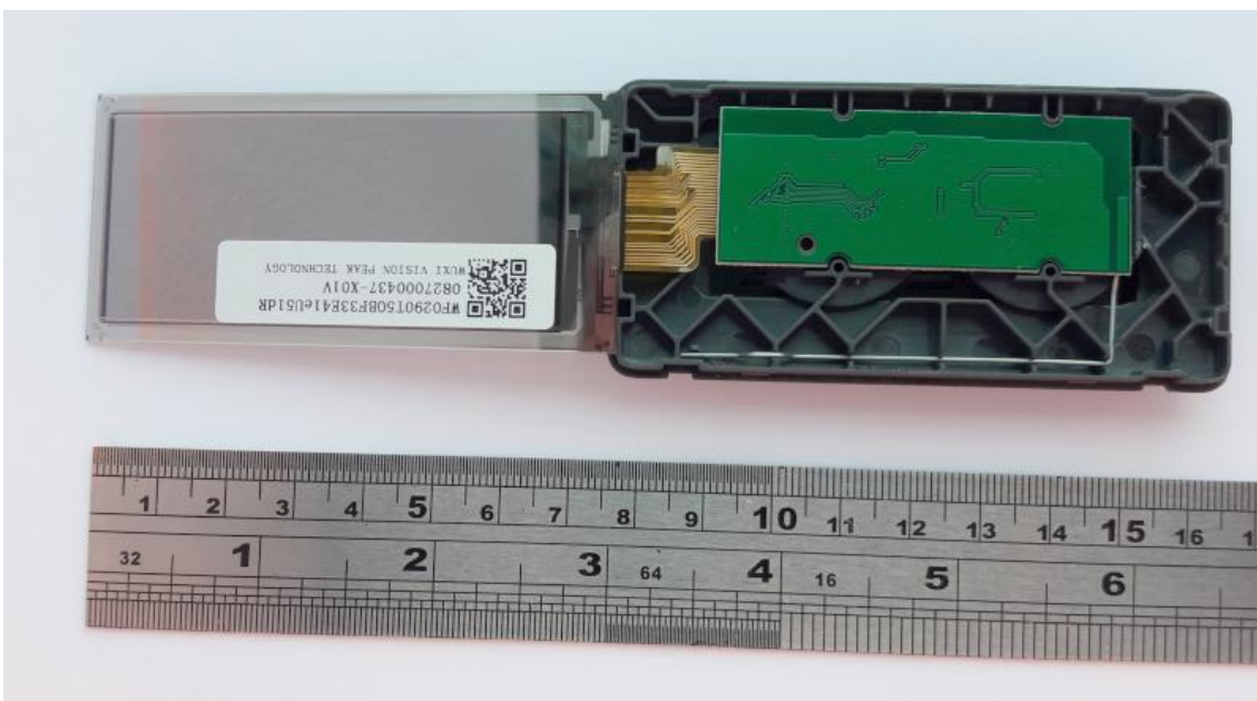
PCB located in rear cover before folding display module over:
