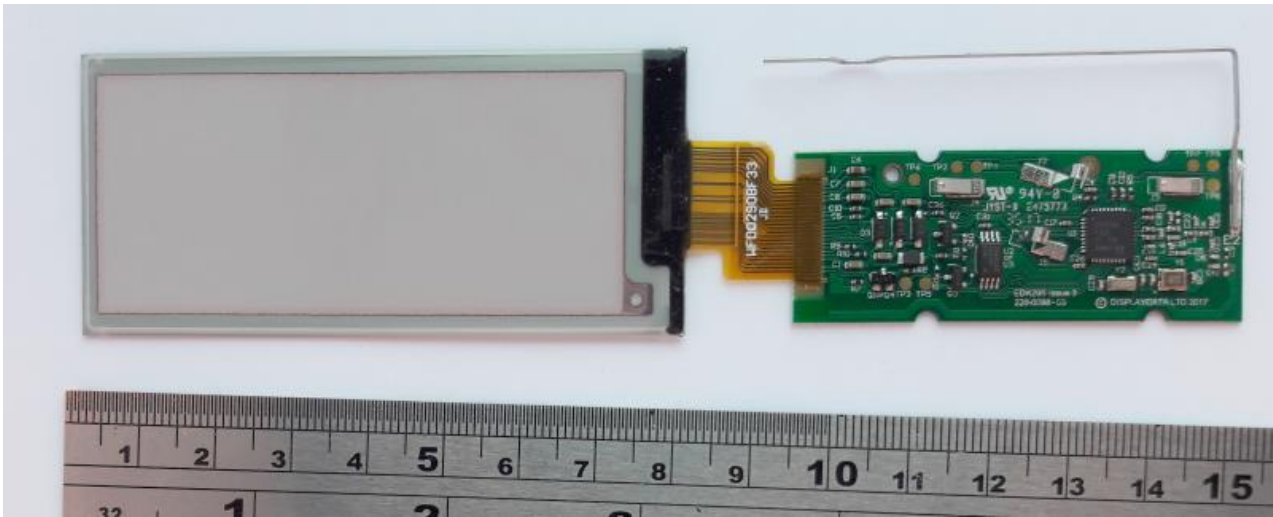
PCB component side with bonded Display and wire antenna:
