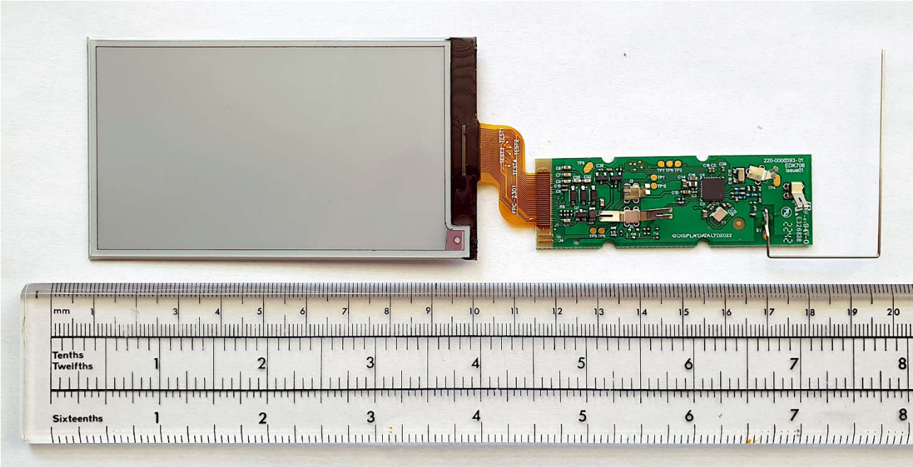
DD29-3A (Chroma 37+) – PCB and display glass front side,
