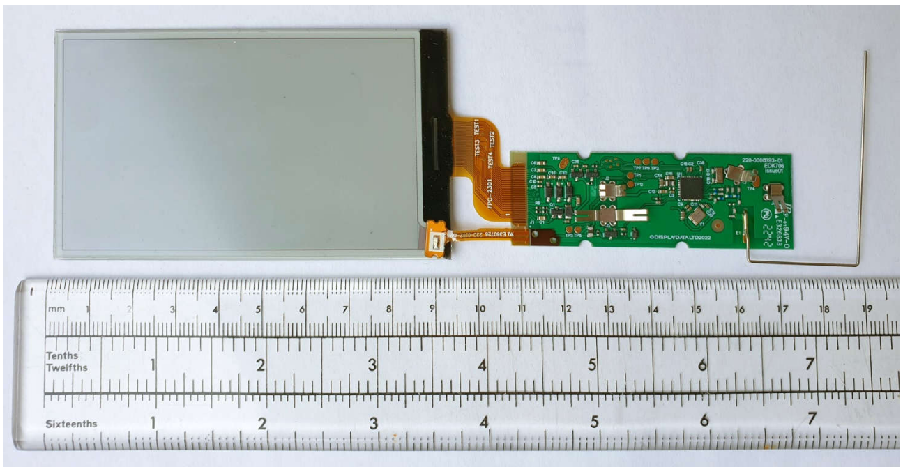
DD37-3A (Chroma 37L) – PCB and display glass front side.
