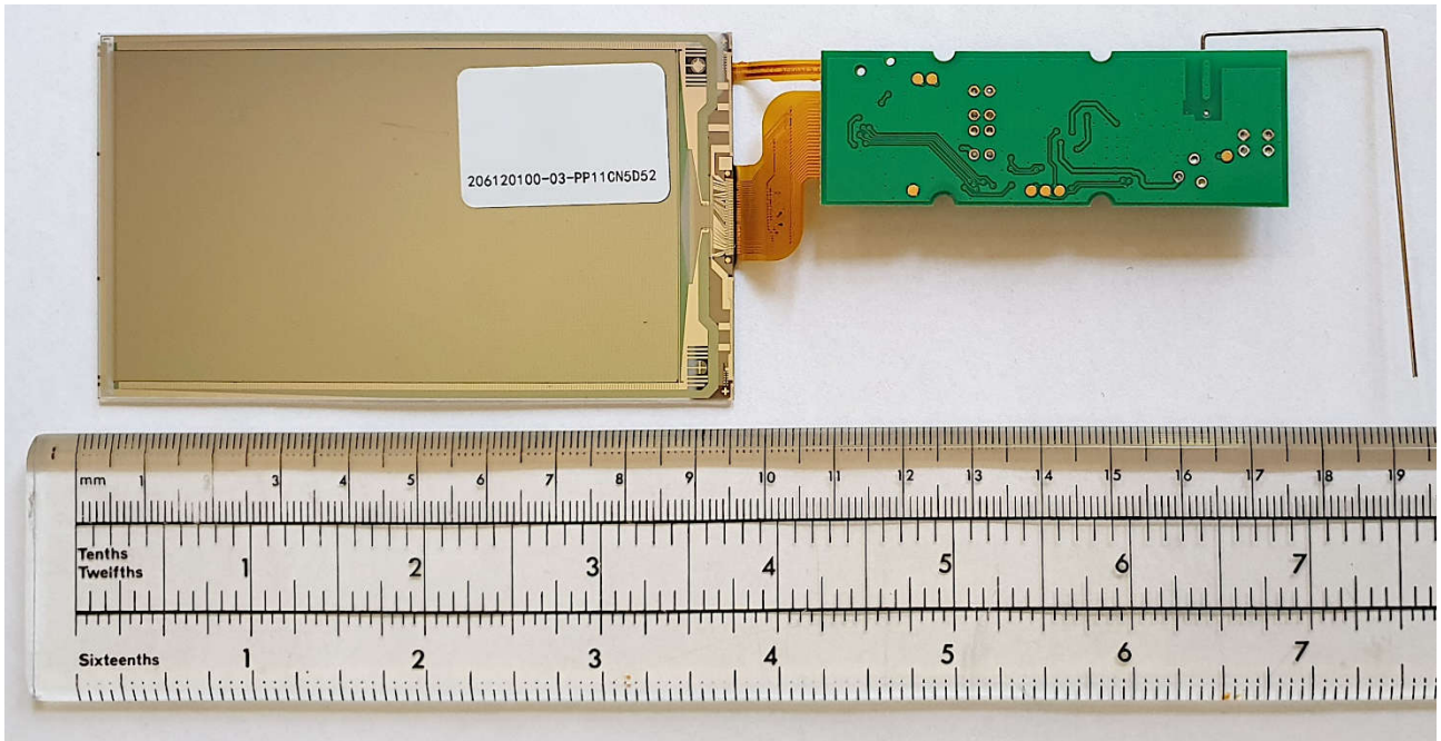
DD37-3A (Chroma 37L) – PCB and display glass rear side.
