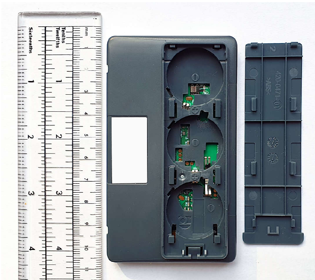
DD37-3A (Chroma 37+) – Battery Cover and Coin cell removed.
