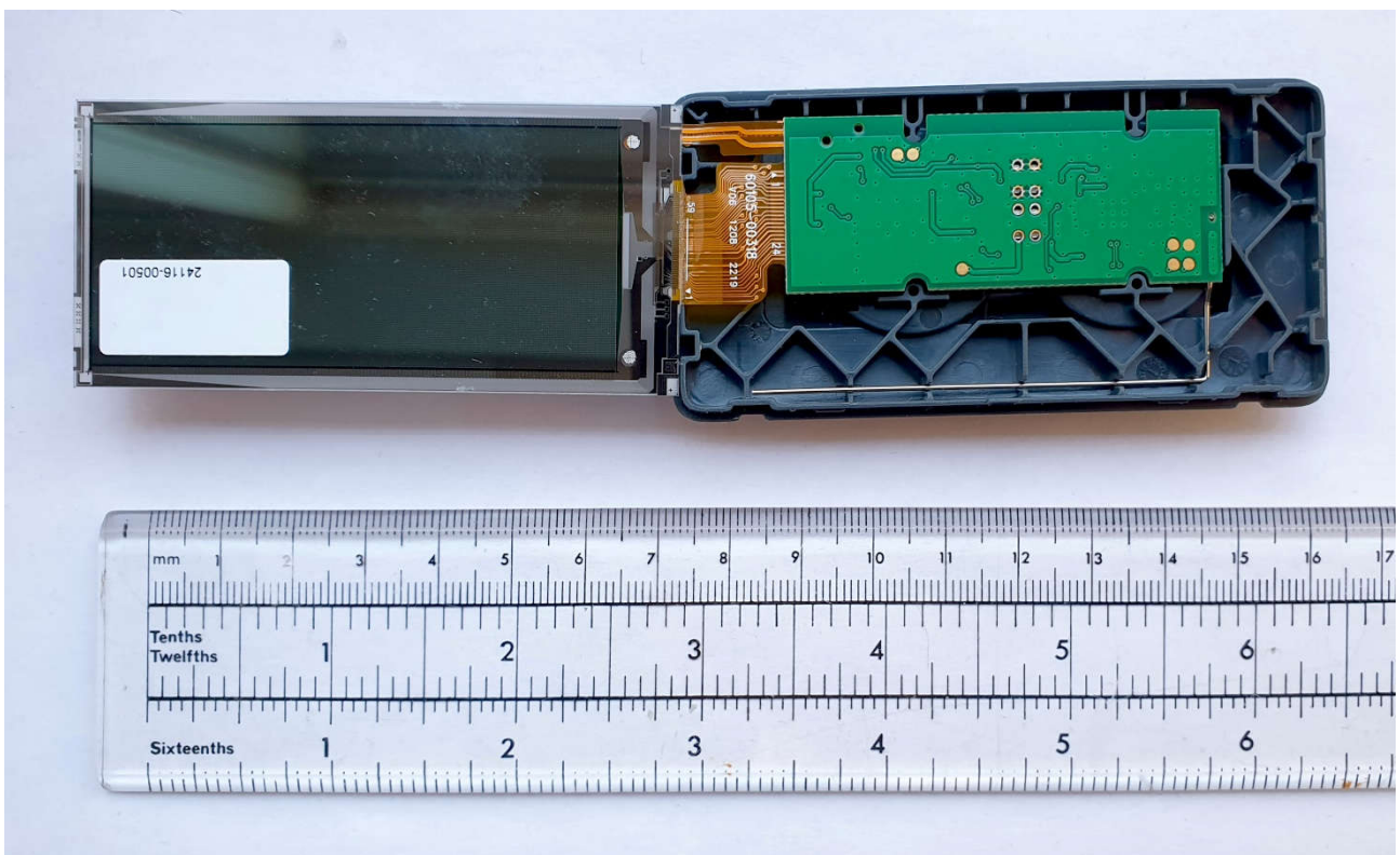
DD29-3A (Chroma 29L) – Front cover removed and display glass folded open.
