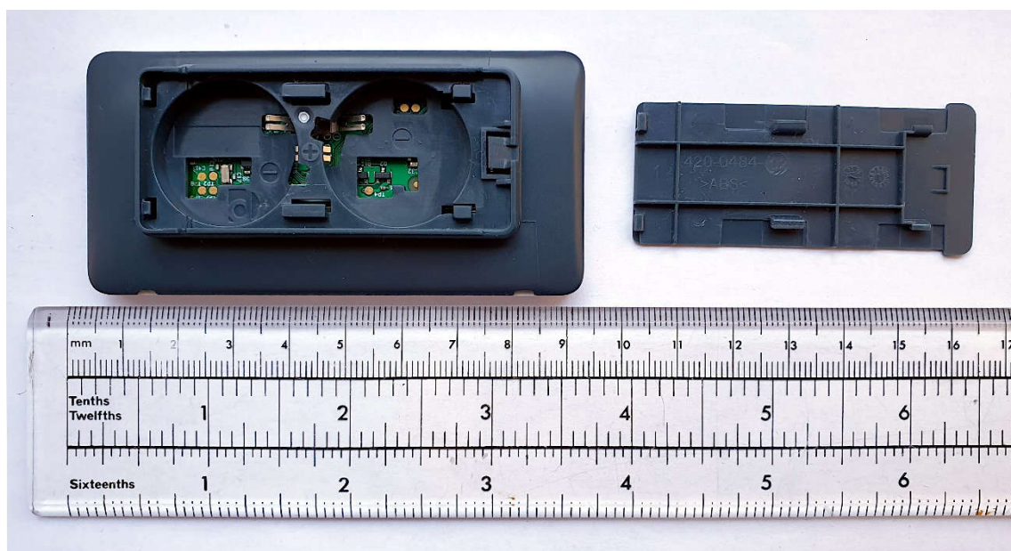
DD29-3A (Chroma 29+, Aura 29F+) –Battery Cover and 2 x CR2450 coin cells removed.
