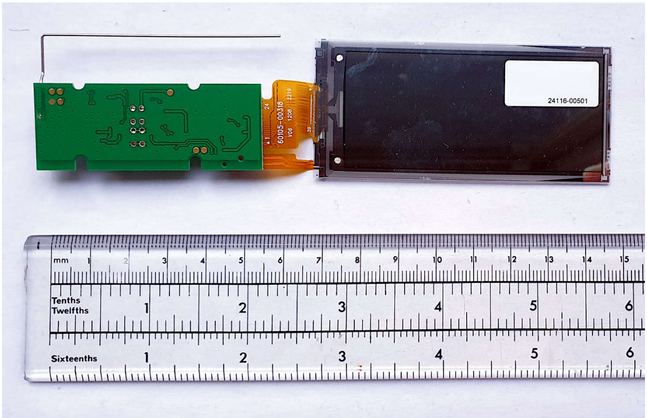
DD29-3A (Chroma 29L) – PCB and display glass rear side
