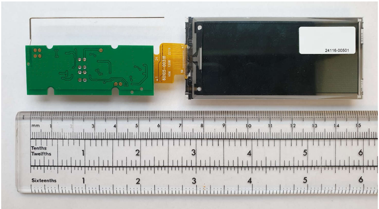
DD29-3A (Chroma 29+, Aura 29F+) – PCB and display glass rear side.
