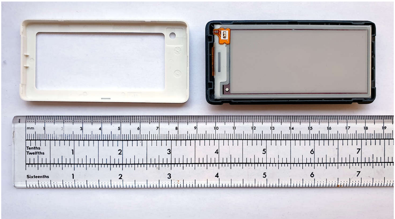
DD29-3A (Chroma 29L) – Front cover removed.
