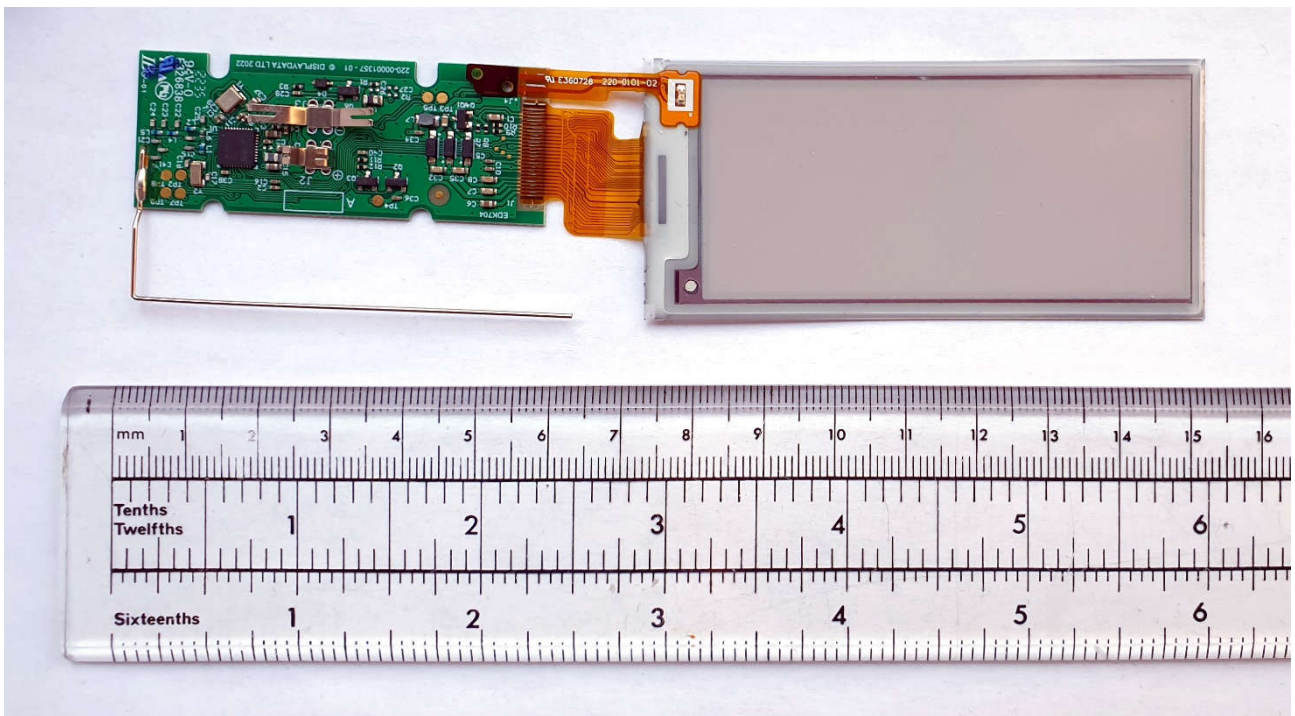
DD29-3A (Chroma 29L) – PCB and display glass front side.
