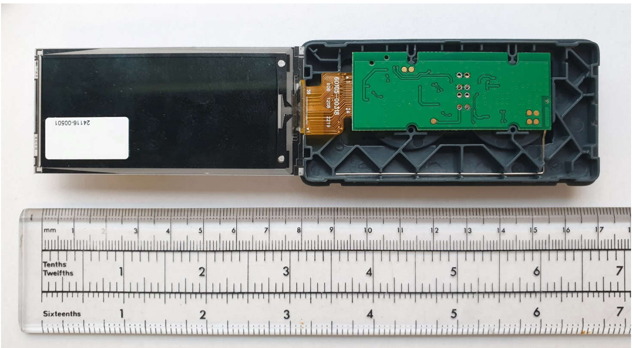
DD29-3A (Chroma 29+, Aura 29F+) – Front cover removed and display glass folded open.
