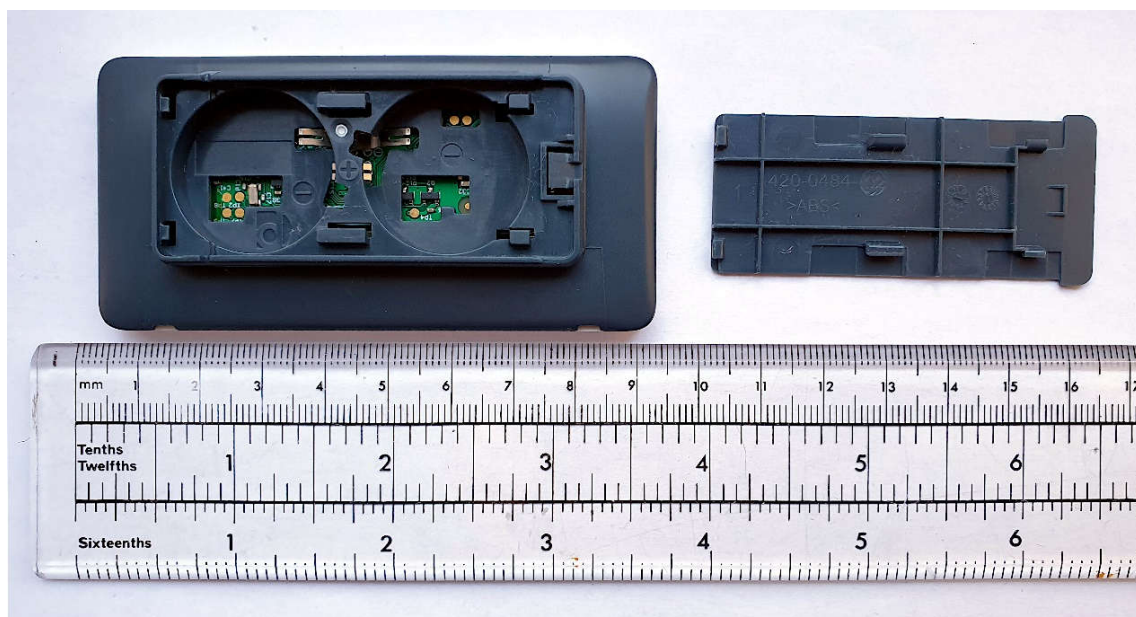
DD29-3A (Chroma 29L) – Battery Cover and 2 x CR2450 coin cells removed.
