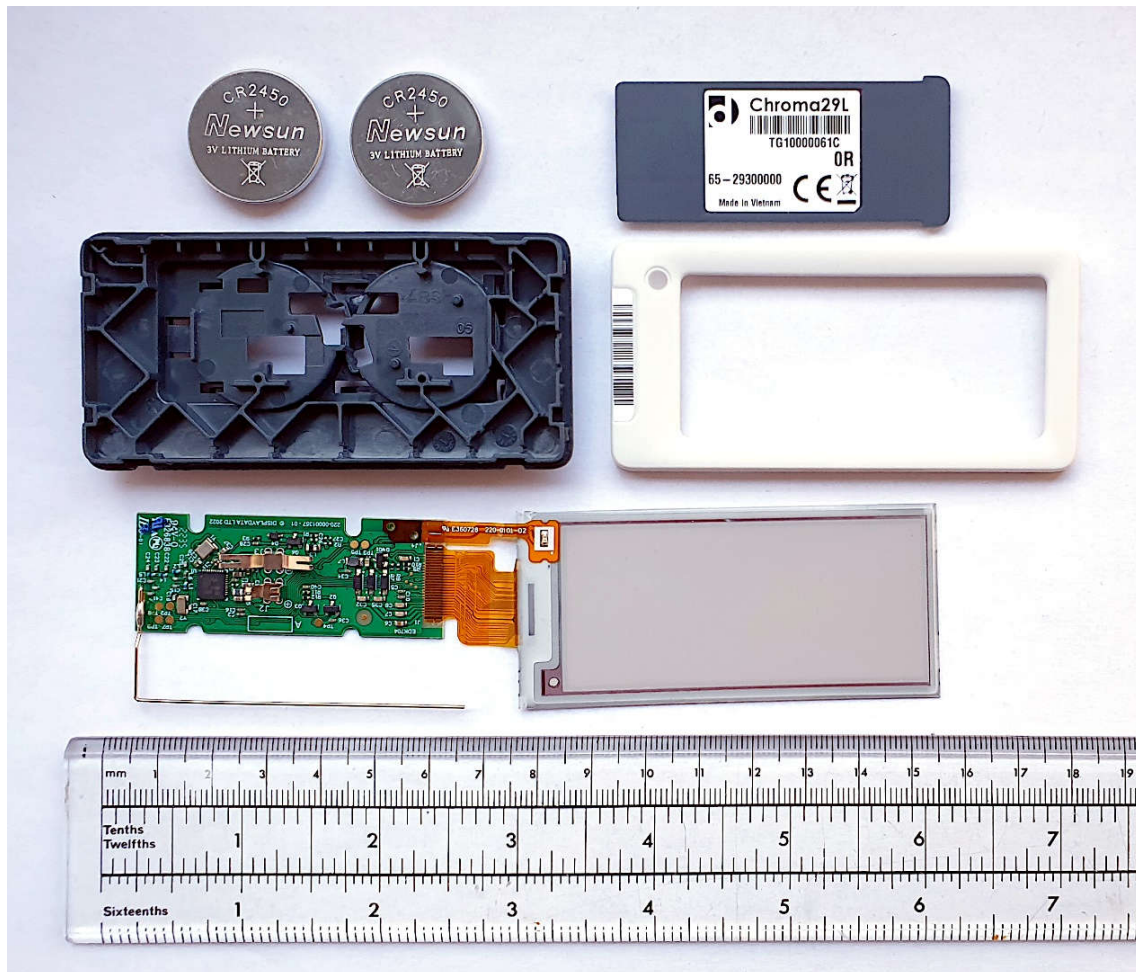
DD29-3A (Chroma 29L) – All components
