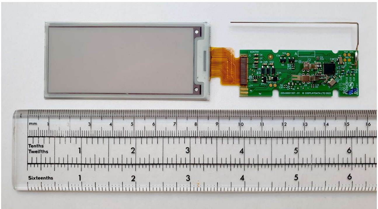
DD29-3A (Chroma 29+, Aura 29F+) – PCB and display glass front side,
