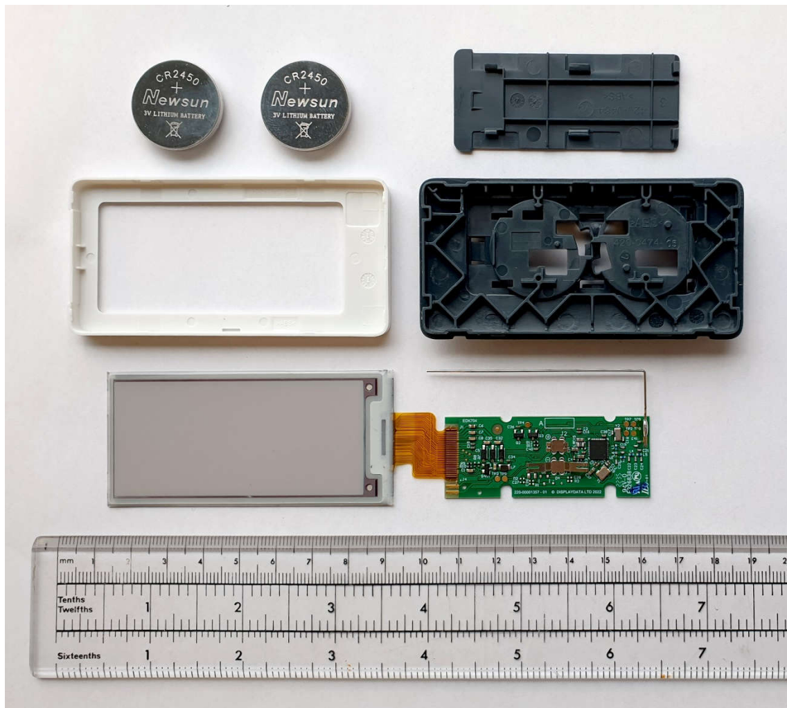
DD29-3A (Chroma 29+, Aura 29F+) – All components
