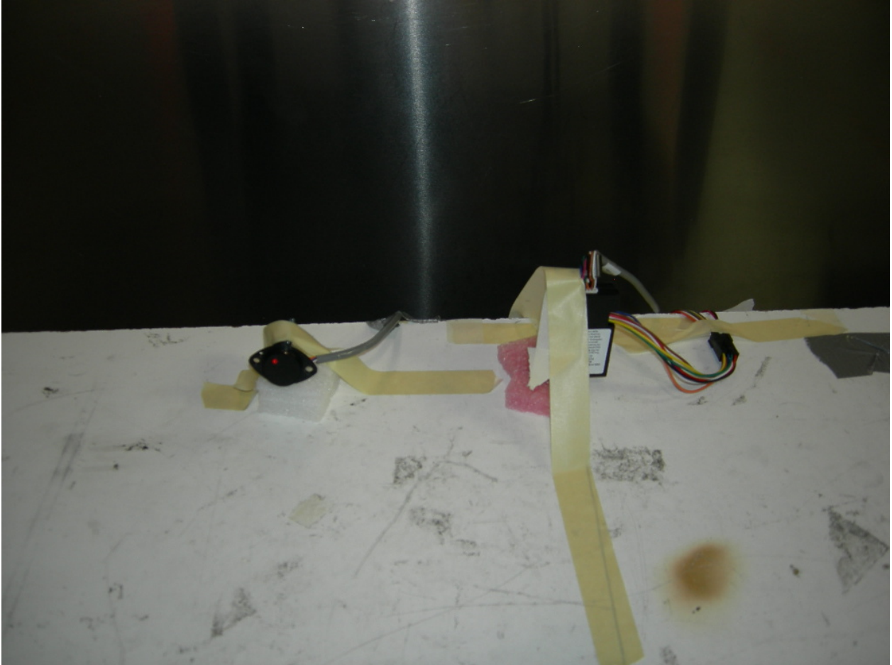
Figure 5: Conducted Emissions
