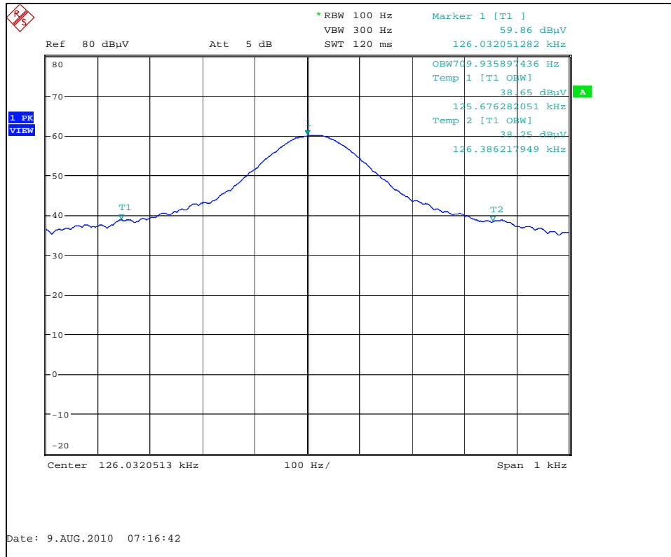
Figure 7.4.2-2: 99% Bandwidth Plot
