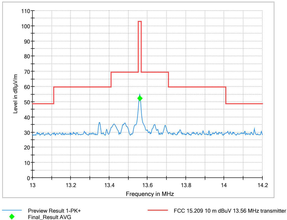
Figure 4.4.1 Field strength of fundamental.
