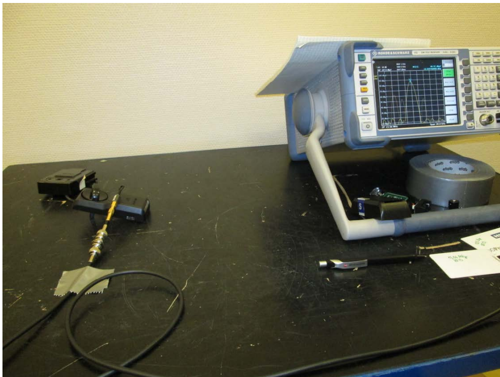
Photo 4.6.1 Test setup regarding measurement of carrier frequency stability.
