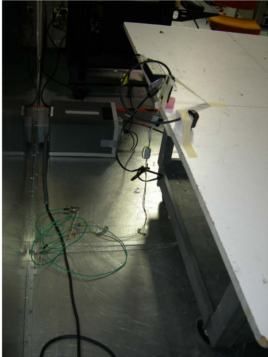
Figure 6: Conducted Emissions
