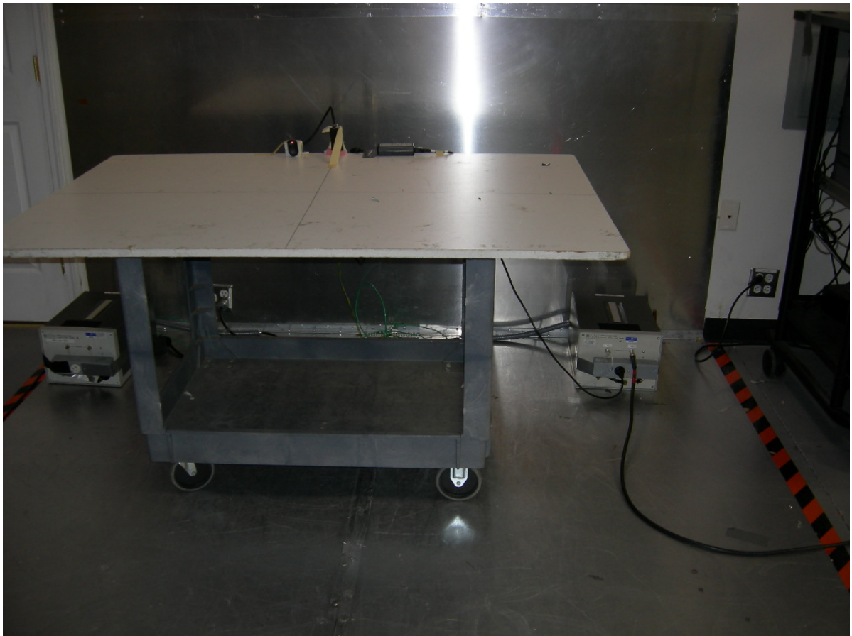
Figure 5: Conducted Emissions
