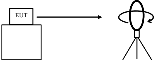
Figure 2: Direction of the Loop Antenna
