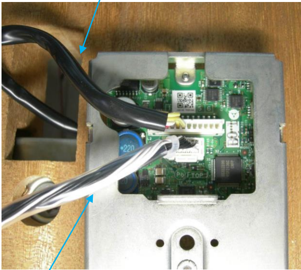
Antenna and Sub board connection
