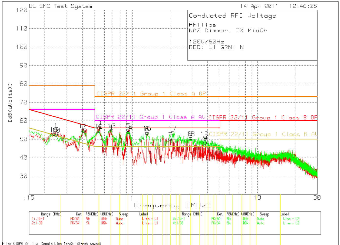
Figure 6 Conducted Emissions Graph – Dimmer – Middle Channel
