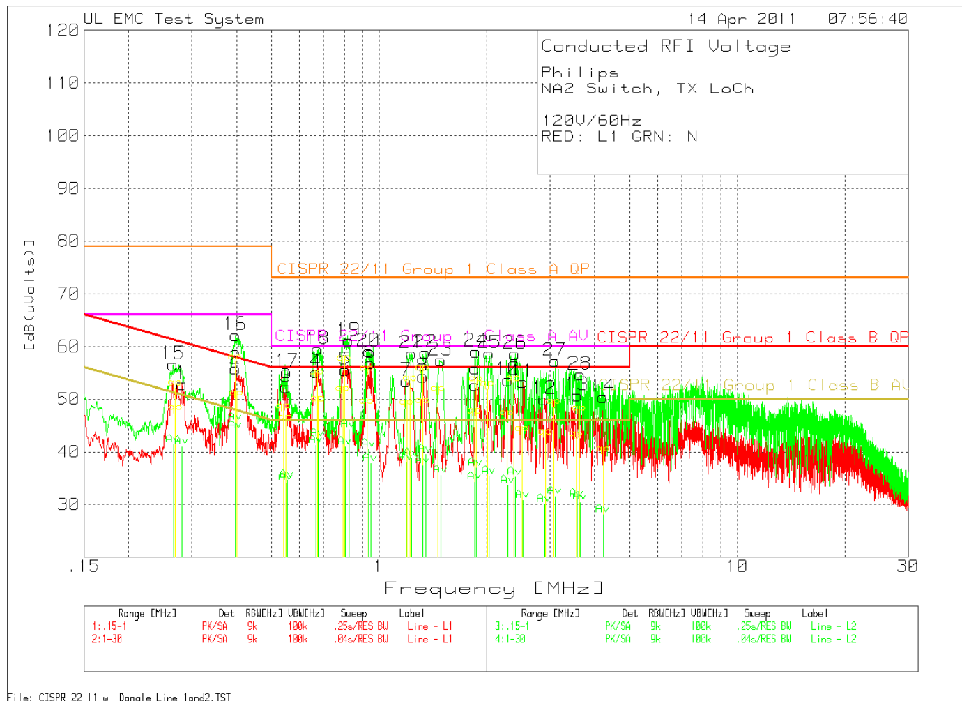
Figure 2 Conducted Emissions Graph – Switch – Low Channel
