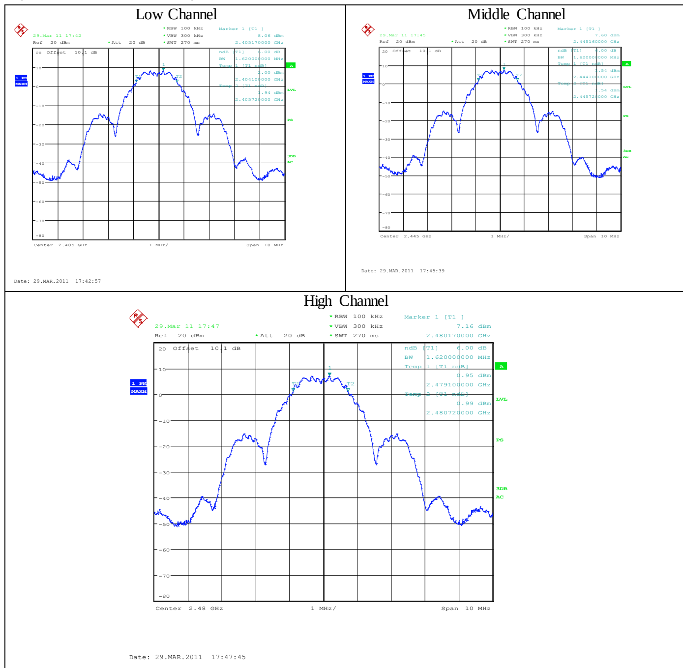
Figure 40 6dB Bandwidth Graphs
