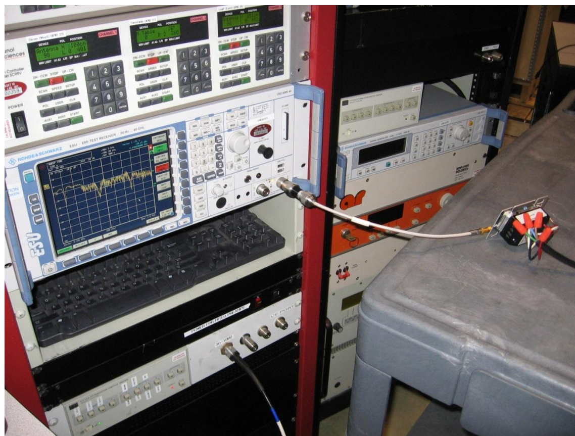
Test Setup for Duty Cycle
