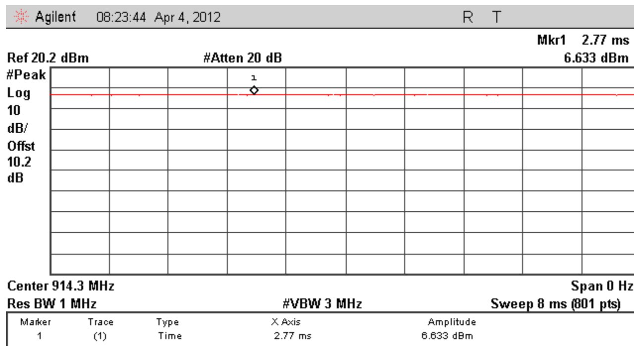
Figure 21 Maximum Peak Output Power Graphs – Mid Channel
