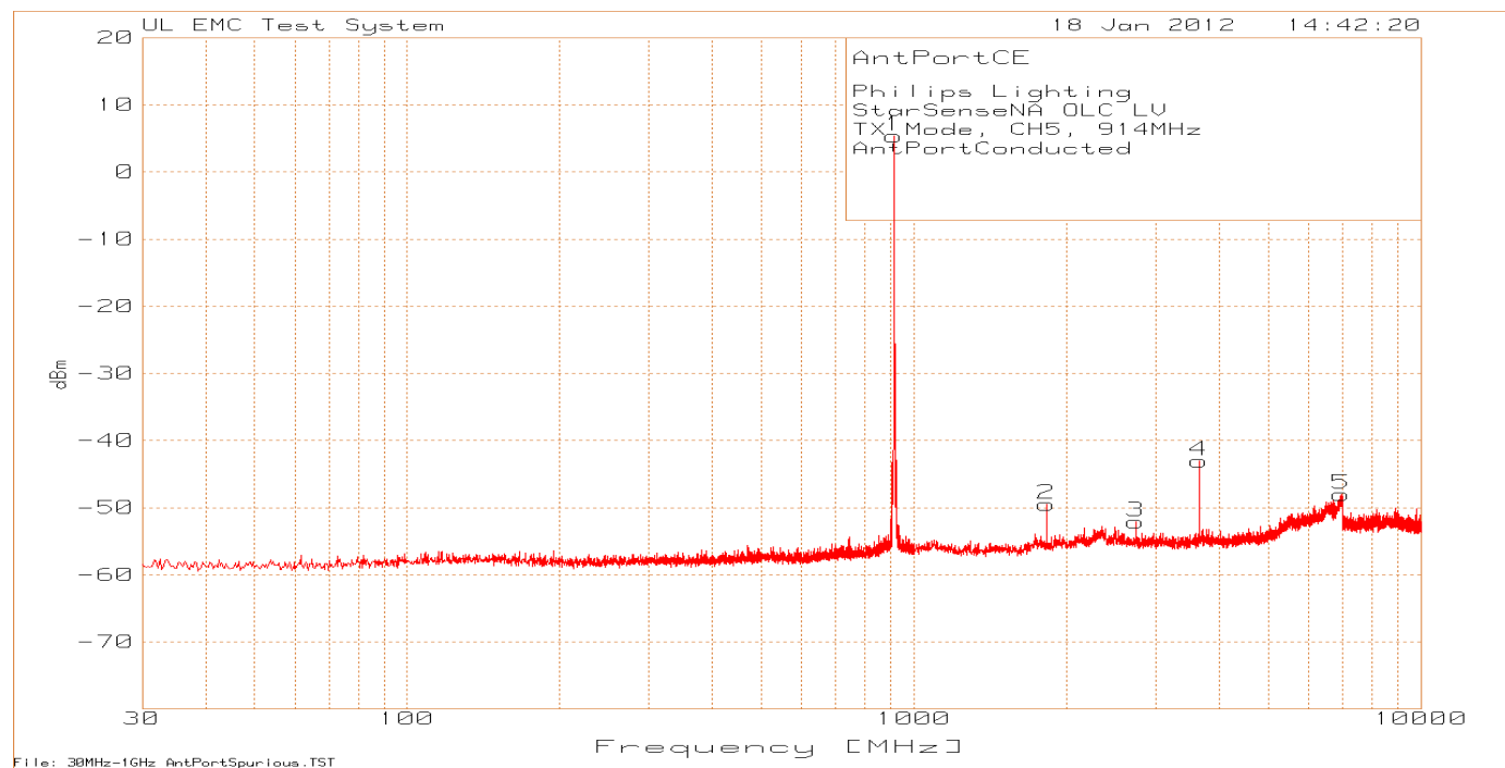
Figure 7 30MHz-10GHz Antenna Port Spurious Emissions Plots TX Mode Middle Channel.
