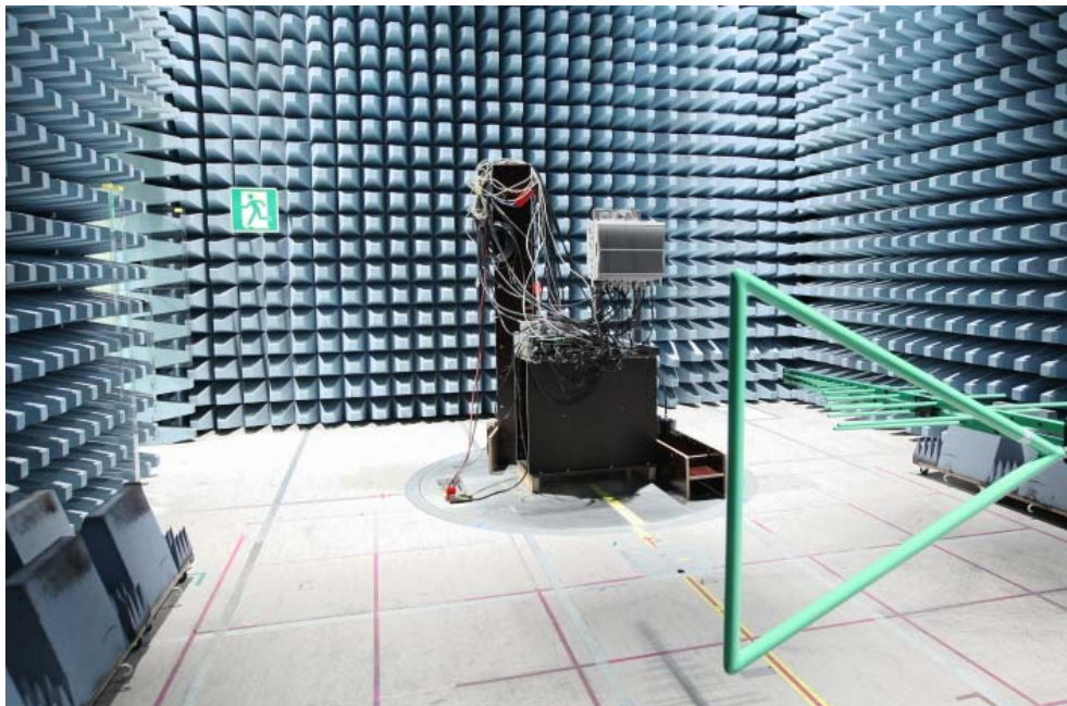
Radiated Emissions- EUT in chamber
