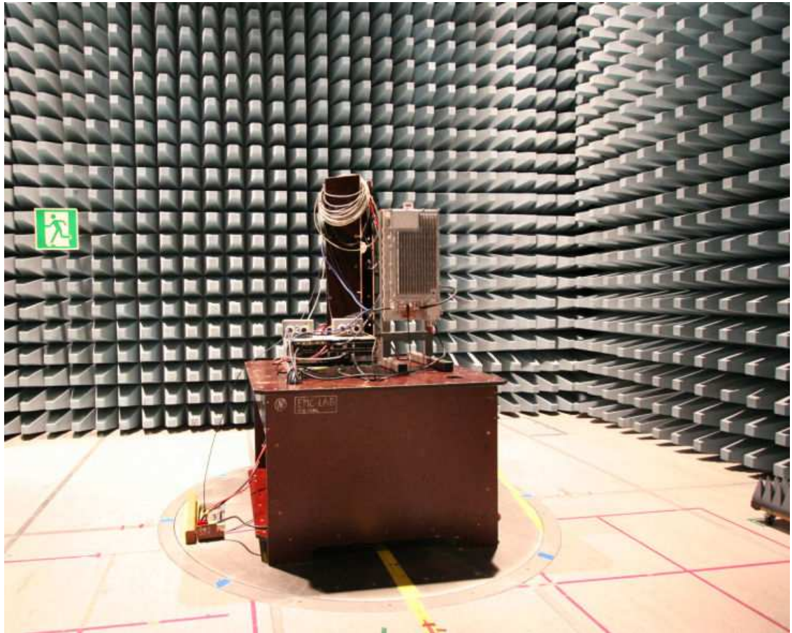
Photograph 1: Radiated spurious emissions test
